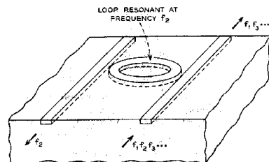
Fig. 1 — Channel dropping filter (ring type).
