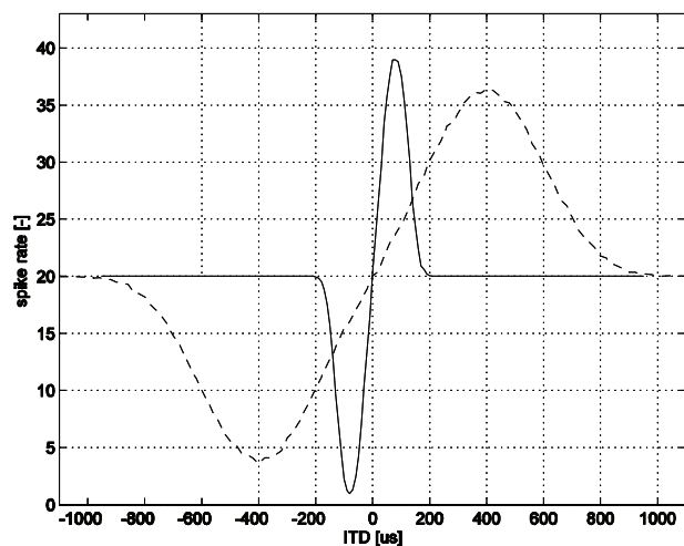
Fig. 5. Effect of the timing jitter magnitude. Two magnitudes of timing jitter \Delta_{tA} and \Delta_{tB} are shown here, 100 \mu\text{s} as a solid line (-) and 400 \mu\text{s} as a broken line (---). They also set the slope of the model output curve and thus the range of ITDs detected. Together with the previous Figure 4, this shows the robustness of the model with respect to variation of parameters. Figures 4 and 5 illustrate the range of parameter values accessible to the model.
