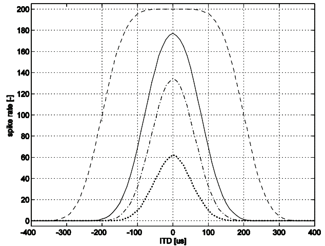
Fig. 4. Effect of the size of the time window. The width of the time windows for CDs sets the range of ITDs detectable by the circuit. Four widths are compared here: \Delta_w = 200 \mu\text{s} (---), 80 \mu\text{s} (-), 50 \mu\text{s} (-.) and 20 \mu\text{s} (...). Plotted output activity is dependent on ITD, as in Figure 3. Only the excitatory part is active in this plot. From an engineering point of view, an optimal curve uses the full dynamic range of available output activities, \Delta_w = 50 \mu\text{s} .
