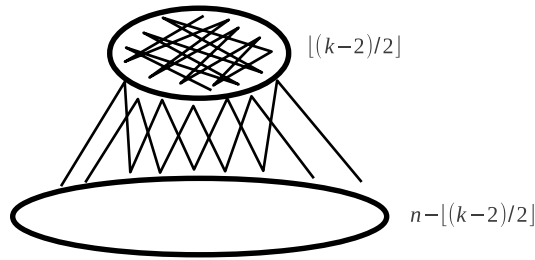
Figure 1.2: An almost extremal graph for the Erdős–Sós Conjecture.
