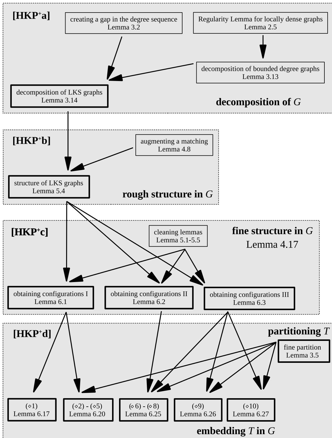
Figure 1.3: Structure of the proof of Theorem 1.3, including parts from [HKP b , HKP c , HKP d ].
