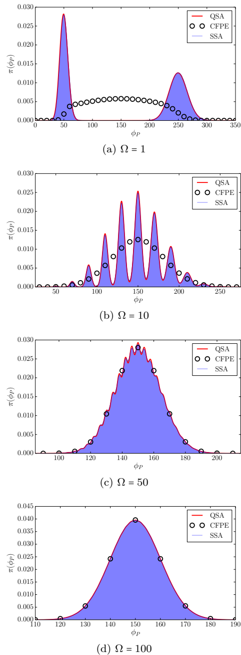
Figure 1: Comparison of the stationary distribution of protein concentration obtained from SSA simulations with the QSA solution \pi(\phi_P) , and the numerical solution of the CFPE for different values of volume, \Omega . Parameters (see text) are such that timescale separation is enforced. The QSA and SSA predict multimodality below a certain volume whereas the CFPE predicts a unimodal distribution for all volumes.
