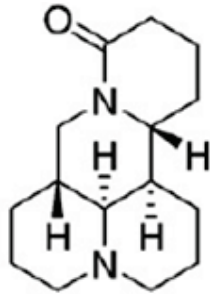
Fig. 1. Chemical structure of sophoridine.
