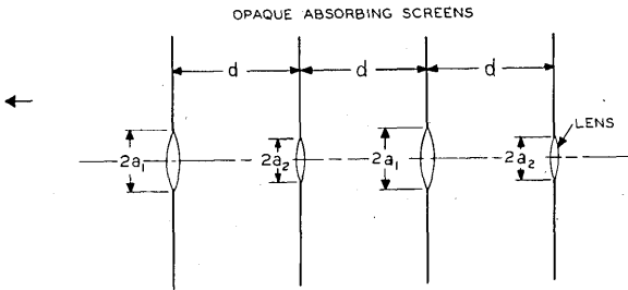
Fig. 16. Geometry of a spherical-mirror resonator with finite mirror apertures and the equivalent sequence of lenses set in opaque absorbing screens.
