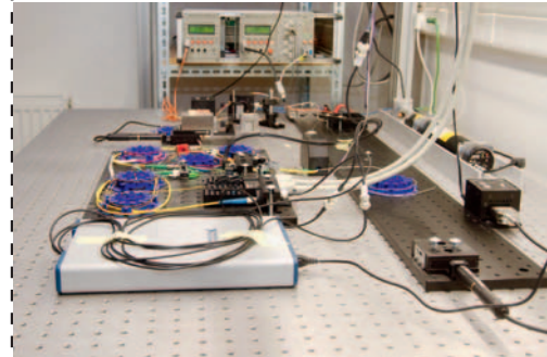
Testbed for fiber-optic displacement sensors based on FBG technology and evaluation through spectrum analysis
