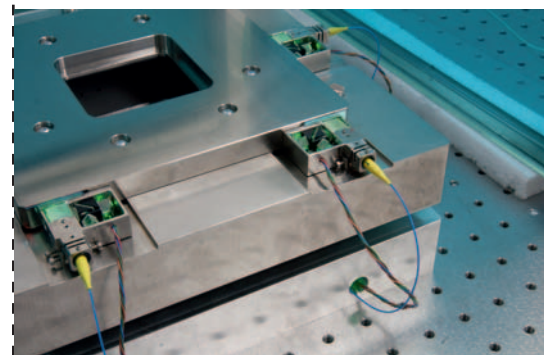
Positioning platform with six-axis interferometric measurement and motion control for nanometrology
