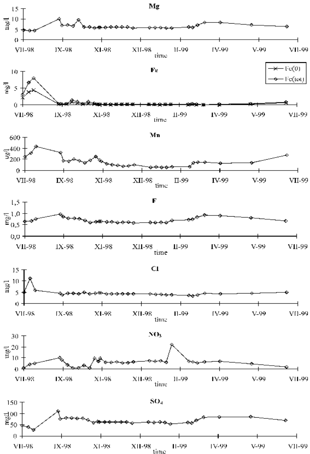
Fig. 22. Seasonal variations of Mg, Fe, Mn, F, Cl, SO 4 , NO 3 at Lesni Brook.
