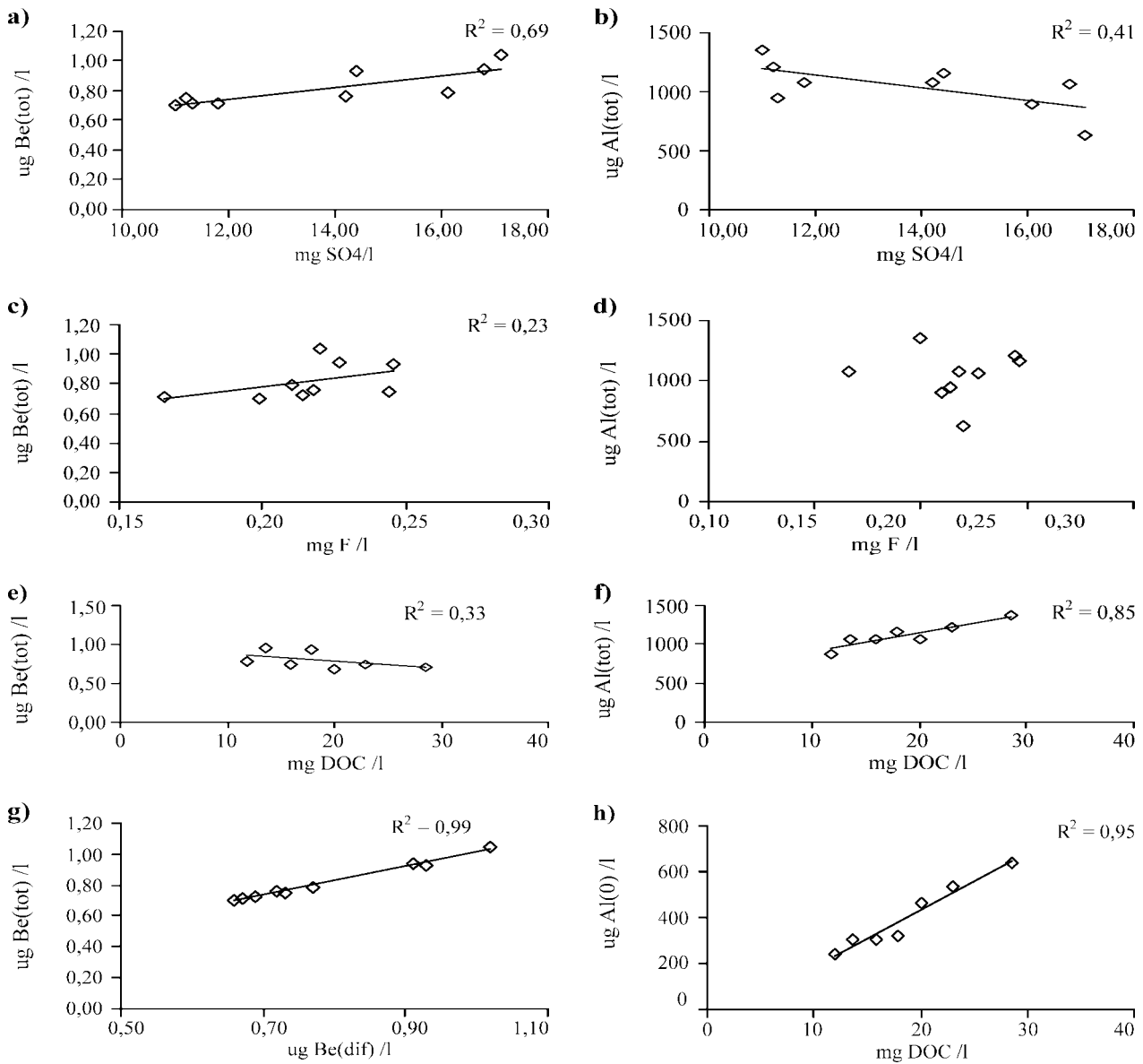
Fig. 12. Relationship of the Be, Al fractions with SO 4 , F, DOC (L).
