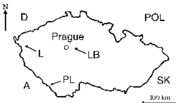
Fig. 1. Location of the sites in Czech Republic.
