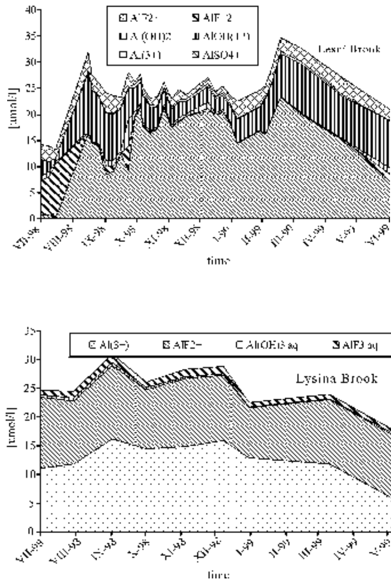
Fig. 23. Seasonal variations of the Al speciation at Lesni Brook and Lysina Brook.
