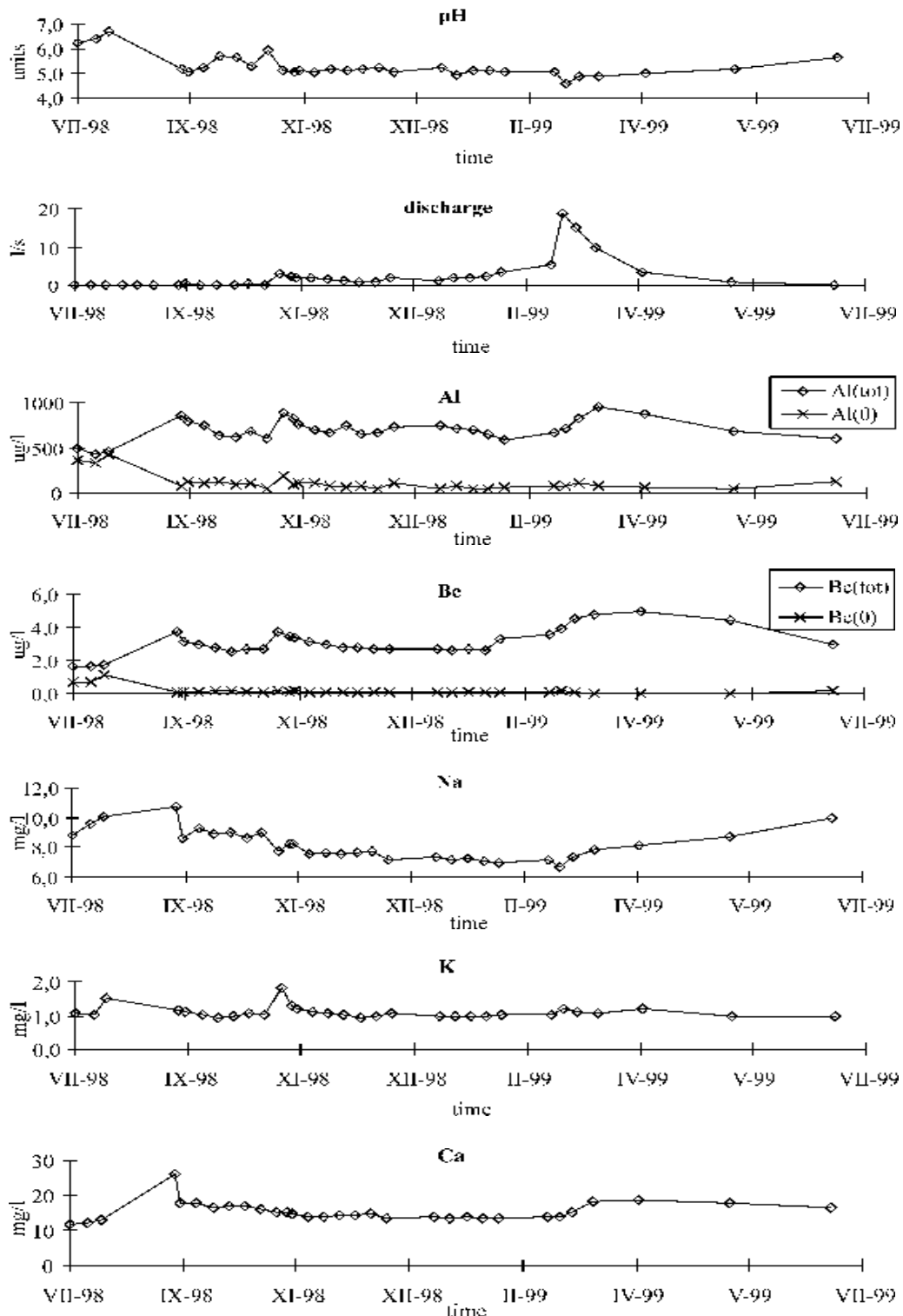
Fig. 21. Seasonal variations of pH, discharge, Al, Be, Na, K, Ca at Lesni Brook.
