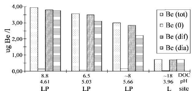
Fig. 13. Be concentration (ug/l) for dialyzed samples.
