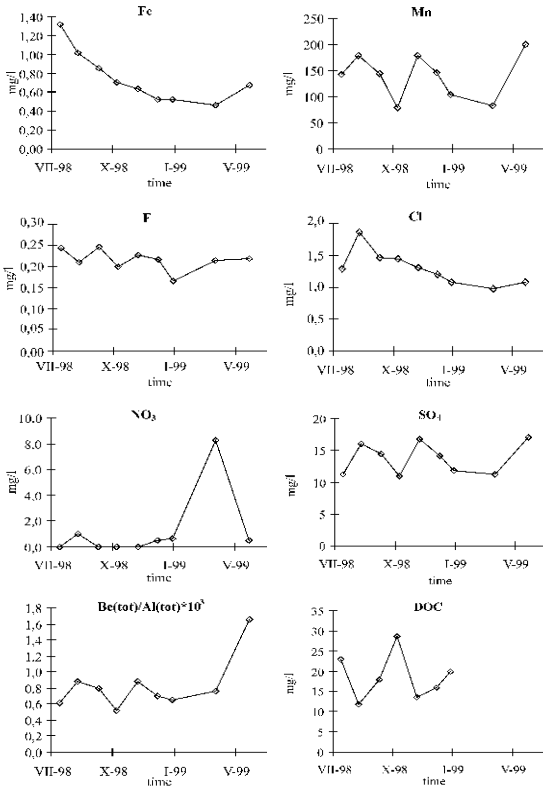
Fig. 20. Seasonal variations of Fe, Mn, F, Cl, NO 3 , SO 4 , Be/Al, DOC at Lysina Brook (DOC data from Hruška and Krám), unpublished data.
