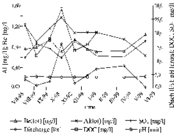
Fig. 4. Seasonal variations of Lysina brook chemistry.
