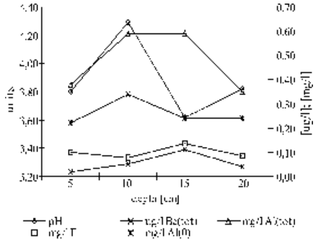
Fig. 5. Variations of pH, F, Be, Al with depth in catchment Lysina soil horizons (L).
