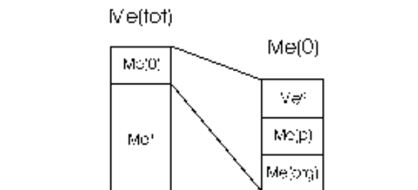
Fig. 2. Element speciation description.
