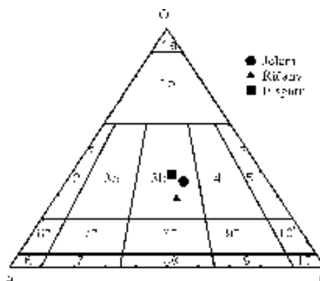
Fig. 14. Positions of studied granites in QAP figure.
