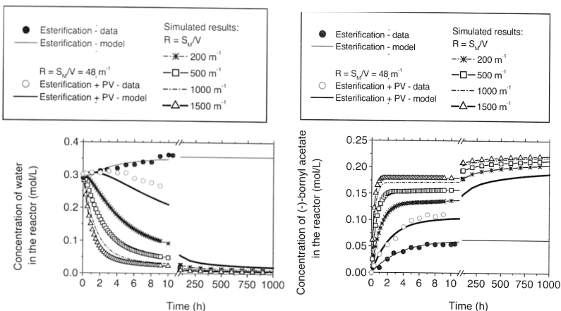
Figure 11. Effect of the S_M/V ratio on the conversion to (–)-bornyl acetate [O13].
