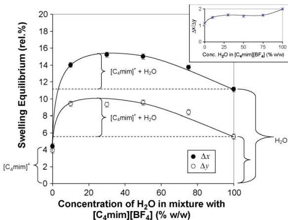
Fig. 5. Swelling equilibrium data of a Nafion membrane exposed to binary mixtures of \text{H}_2\text{O} and [\text{C}_4\text{mim}][\text{BF}_4] at 25^\circ\text{C} . “ y ” corresponds to the membrane casting direction [O8].
