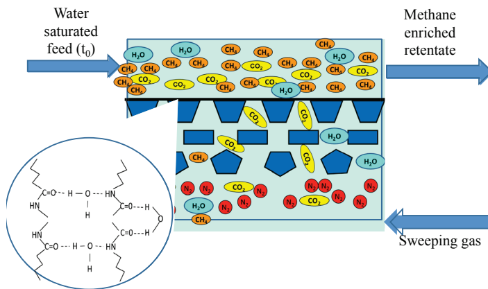
Figure 18. Scheme of function of condensing water membrane on thin film composite reverse osmosis membrane [O22].
