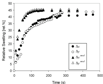
Fig. 9. Swelling kinetics of PU/PBDO membranes and surface-modified PU/PBDOUV membranes in hexyl acetate at T = 25^{\circ}\text{C} (swelling in the transverse casting direction ( \Delta x ) and in the casting direction ( \Delta y ) [O12].
