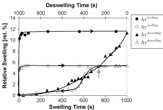
Fig. 6. Anisotropic swelling and “deswelling” kinetics of a Nafion membrane in \text{H}_2\text{O} at 25^\circ\text{C} . “ y ” corresponds to the membrane casting direction [O8].
