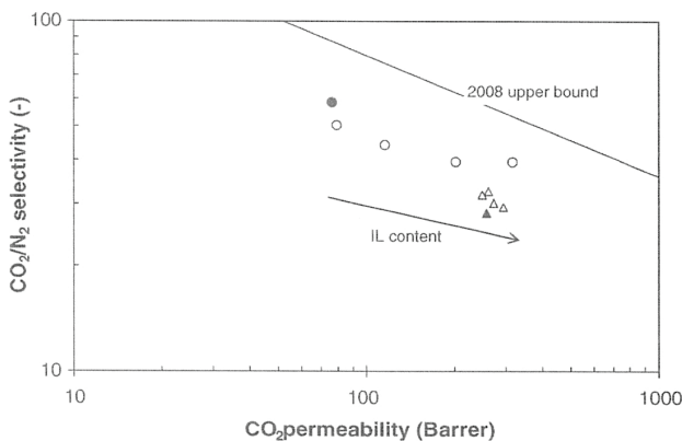
Figure 15. Robeson diagram for the CO 2 /N 2 pair and the IL blend membranes based on Pebax®2533 ( \Delta ), and Pebax®1657 ( \circ ). Filled symbols represent the pure polymer.
