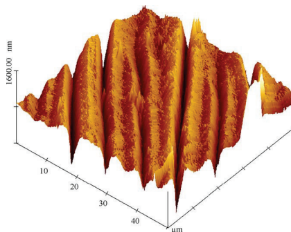
Fig. 10. AFM topography image ( 50\mu\text{m}\times 50\mu\text{m} scan with an image surface area of 2598\mu\text{m}^2 ) of a modified PU/PBDO-UV membrane after a pervaporation experiment. [O12].
