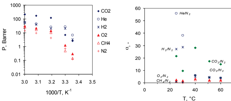
Figure 16. Dependence of permeability (left) and the corresponding permselectivity (right) of six permanent gases as a function of the IL mixture content and temperature (40 wt% of the [EMIM][Tf 2 N]/[HdMIM][Tf 2 N] mixture) [O18].
