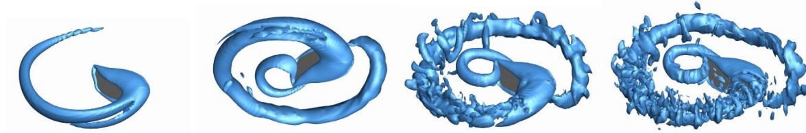
Vortical structures behind the rotating wing of a fruit fly at four different velocities. Figure: The Institute of Mathematics of the CAS
