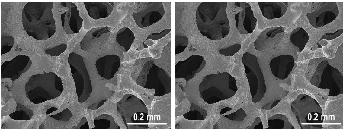
The structure of porous bioglass with composite coating (left).
