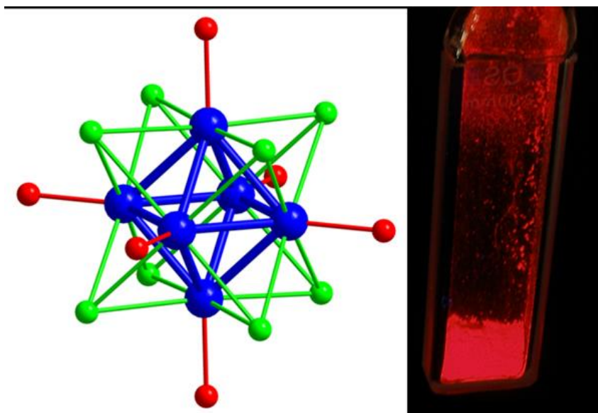
Hexanuclear Molybdenum Clusters: a cluster structure (left) and red luminescence (right). Figure: The Institute of Inorganic chemistry of the CAS
