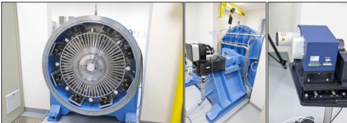
From the Laboratory of Rotational Laser Vibrometry. Photo: The Institute of Thermomechanics of the CAS.
