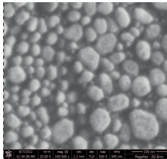
Image of gold on carbon test specimen at the landing energy of 20 eV
