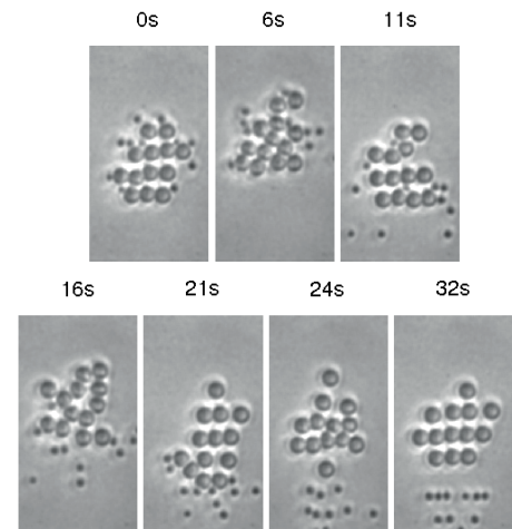
Example of optical sorting of suspension of polystyrene particles of sizes 800 nm and 1600 nm in travelling interference fringes.
