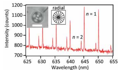
WGM spectra from thermally tuned optically trapped liquid crystal droplet resonator. Scale bar: 10 \mu\text{m}
