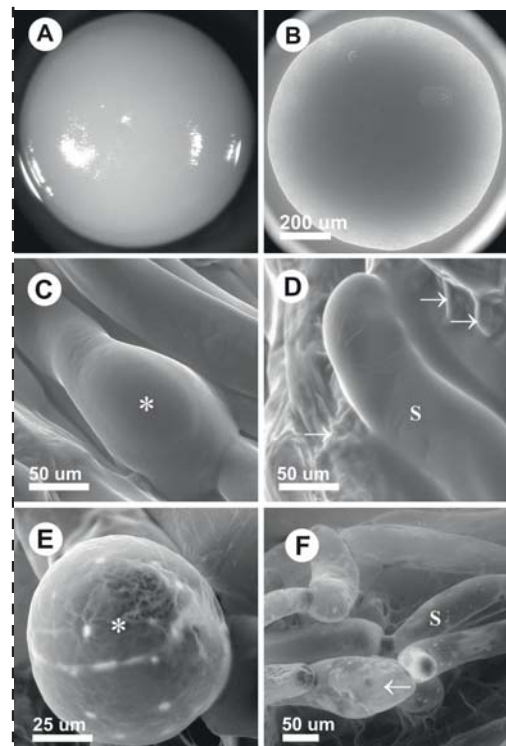
Polymer beads with immobilized cells of recombinant E. coli (10 wt%) with overproduced enzyme cyclopentanone monooxygenase. A) light microscope; B) the ESEM AQUASEM II, with the ionization detector, water vapor pressure 684 Pa, stage temperature 2°C, relative humidity 97%. The embryonic tissue of Picea abies . C,D: observed in commonly used method in ESEM (5°C, 930 Pa water vapor pressure) and E,F: observed using our newly developed Low Temperature Method for ESEM (-20°C, 400 Pa air). S – suspensor cell, arrow – extracellular matrix, *embryogenic head.
