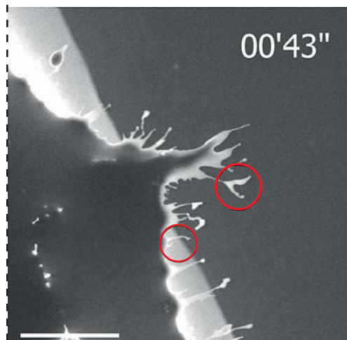
Formation of brine „fingers” during slow evaporation of water from the frost flower. The individual fingers bending and flapping around are highlighted in circles; Imaged with the Environmental Scanning Electron Microscopy (ESEM) AQUASEM II.
