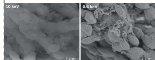
Structure of a mesoporous silica-based nanocomposite as a carrier of catalytic gold nanoparticles, imaged with a standard scanning electron microscope (left image) and by means of low energy electrons (right images).
