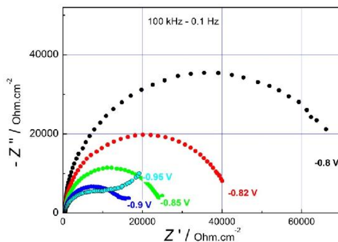
Fig. 4. EIS of 2.5 \times 10^{-4} M ioxynil in dimethylsulfoxide with 0.1 M TBAPF 6 supporting electrolyte at potentials indicated at each curve.
