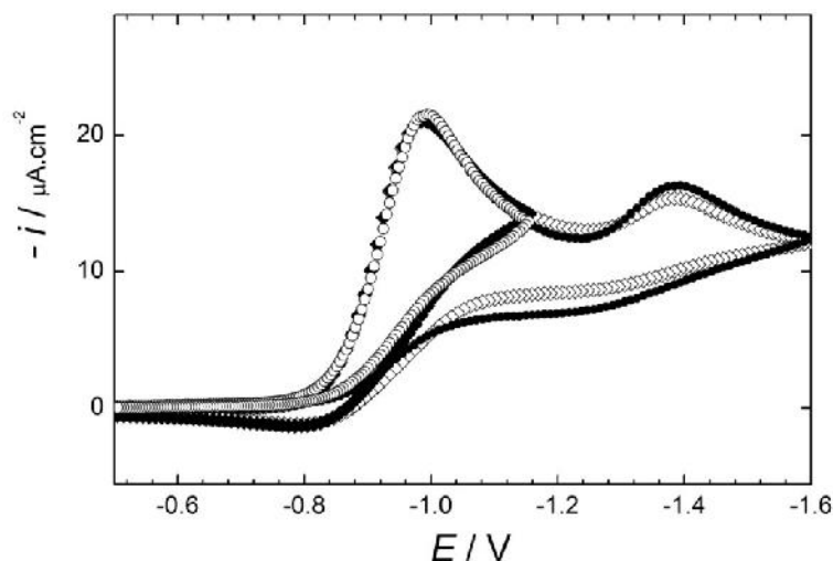
Fig. 3. Cyclic voltammogram of 2.5 \times 10^{-4} M ioxynil in dimethylsulfoxide with 0.1 M TBAPF 6 supporting electrolyte at 0.2 \text{ V}\cdot\text{s}^{-1} . Experimental data are circles and diamonds are results of the numerical fitting.
