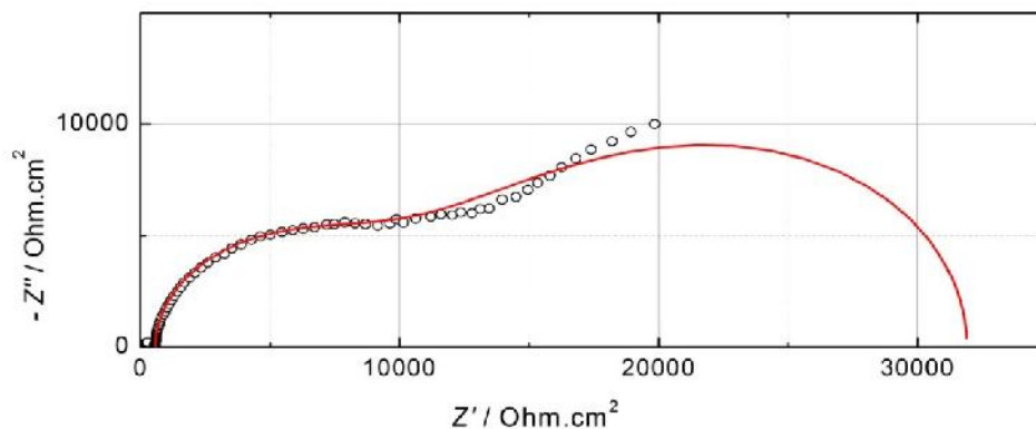
Fig. 7. Diagram of the experimental complex electrode impedance at -0.950 V (circles). Data were fitted with the Gerischer-type circuit resulting in the solution resistance 568 \text{ Ohm.cm}^{-2} , R_{ct}=8057 \text{ Ohm.cm}^{-2} , the double layer capacitance 6.23 \mu\text{F.cm}^{-2} , Y_0=9.79 \times 10^{-5} \text{ S.cm}^{-2} and k = 0.195 \text{ s}^{-1} . Simulation using these parameters and the frequency range from 1 mHz to 30 kHz is shown as the red curve.
