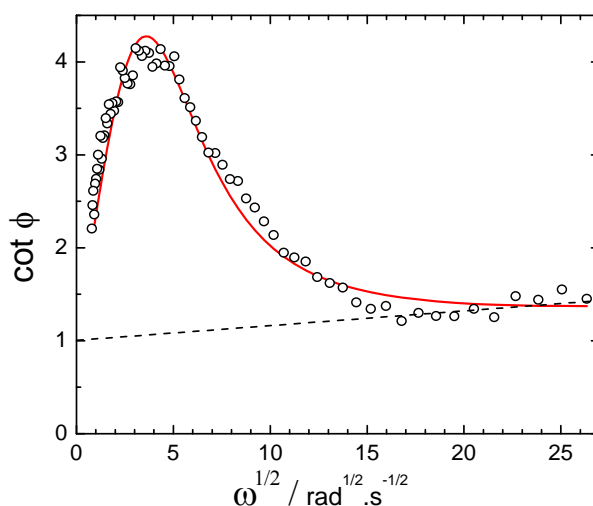
Fig. 8. The experimental dependence of the faradaic phase angle on the applied frequency. The DC potential was -0.95 V. Simulation (full red curve) according to Moreira-De Leve equations used the following values: k(E)=0.157 estimated from the dashed asymptote, k_f=76 , k_{-f}=3.8 , K_f=20.0 and \alpha=0.5 .
