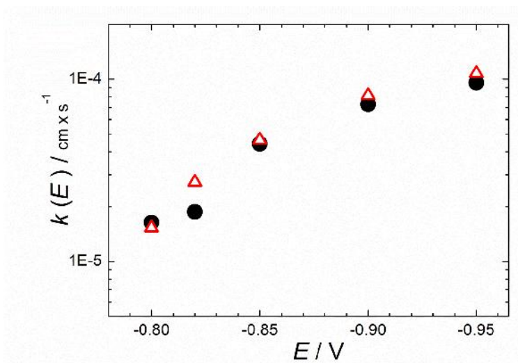
Fig. 6. The heterogeneous rate constant k(E) estimated from the charge transfer resistance for two concentrations of ioxynil: ( \bullet ) 1.9 \times 10^{-4} \text{ M} and ( \Delta ) 2.5 \times 10^{-4} \text{ M} .
