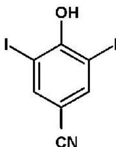
Fig.1. The chemical structure of ioxynil, 4-hydroxy-3,5-diiodobenzonitrile.
