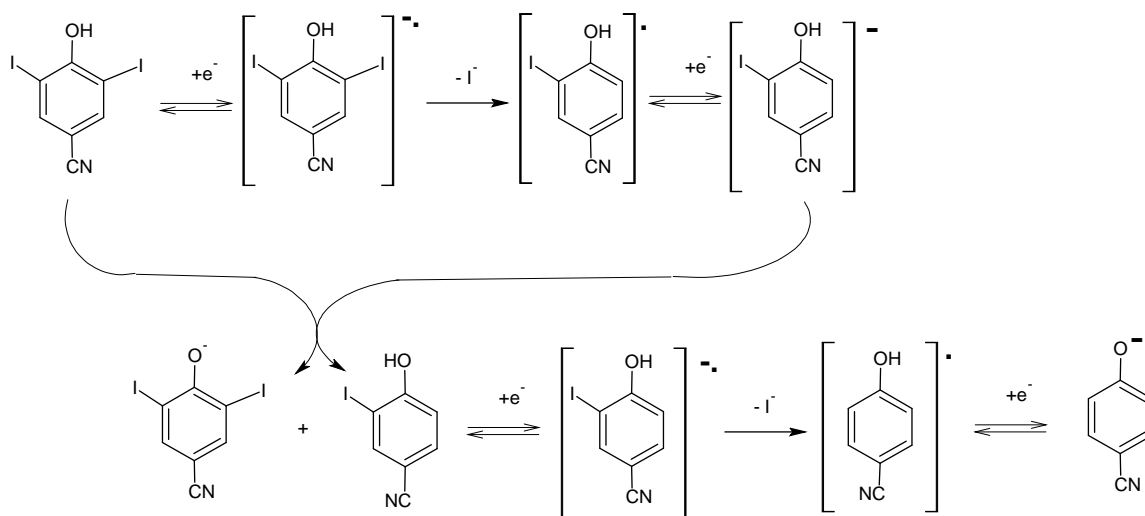
Fig. 2. Mechanism of ioxynil reduction.
