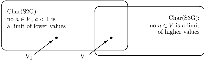
Figure 1: Characteristic classes of S2G, S3G, and PG
