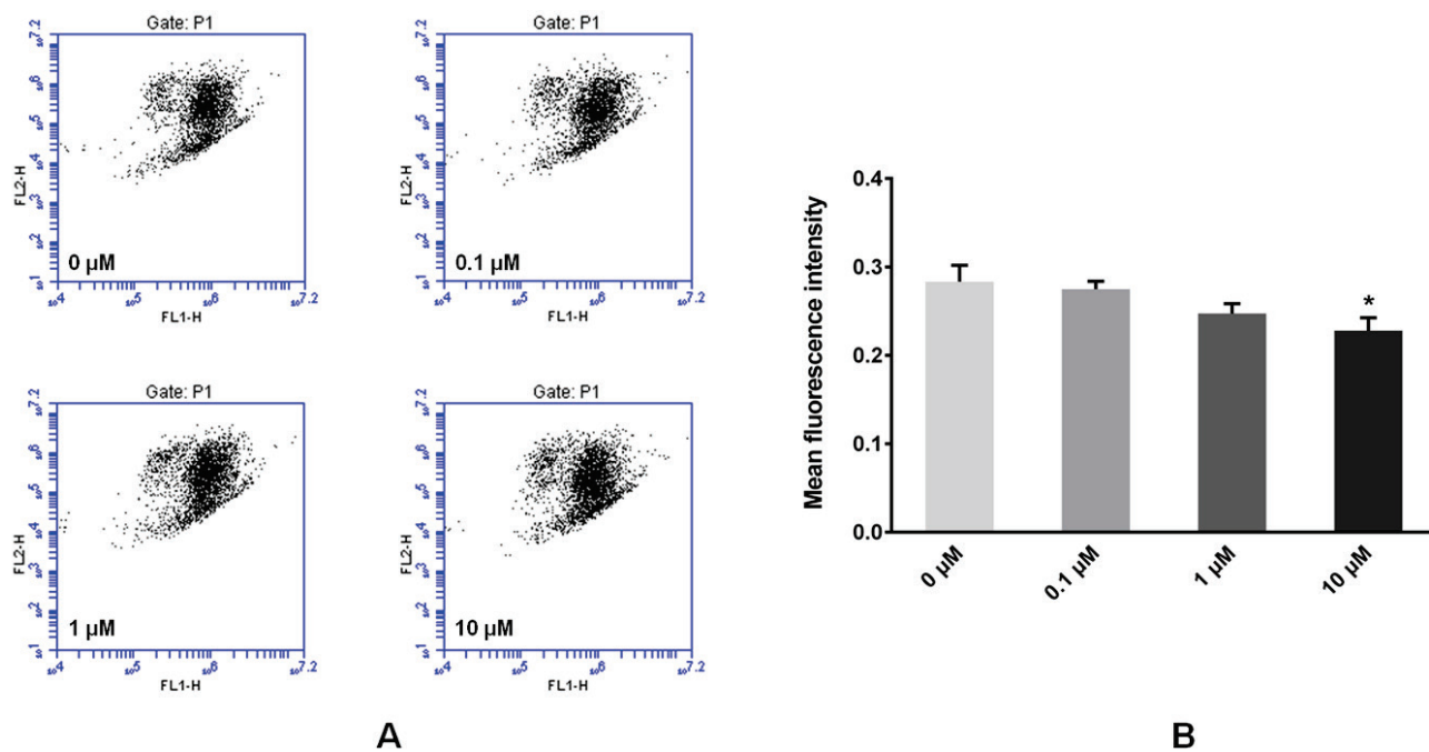
Fig. 6. Effect of DHEA on mitochondrial permeability in primary chicken hepatocytes. (A) Typical mitochondrial permeability images from chicken hepatocytes treated with DHEA. (B) The mitochondrial membrane potential as indicated by the 590/530 nm fluorescence intensity ratio. Data are presented as means \pm SE. * P < 0.05 , DHEA treated group vs. control group.
