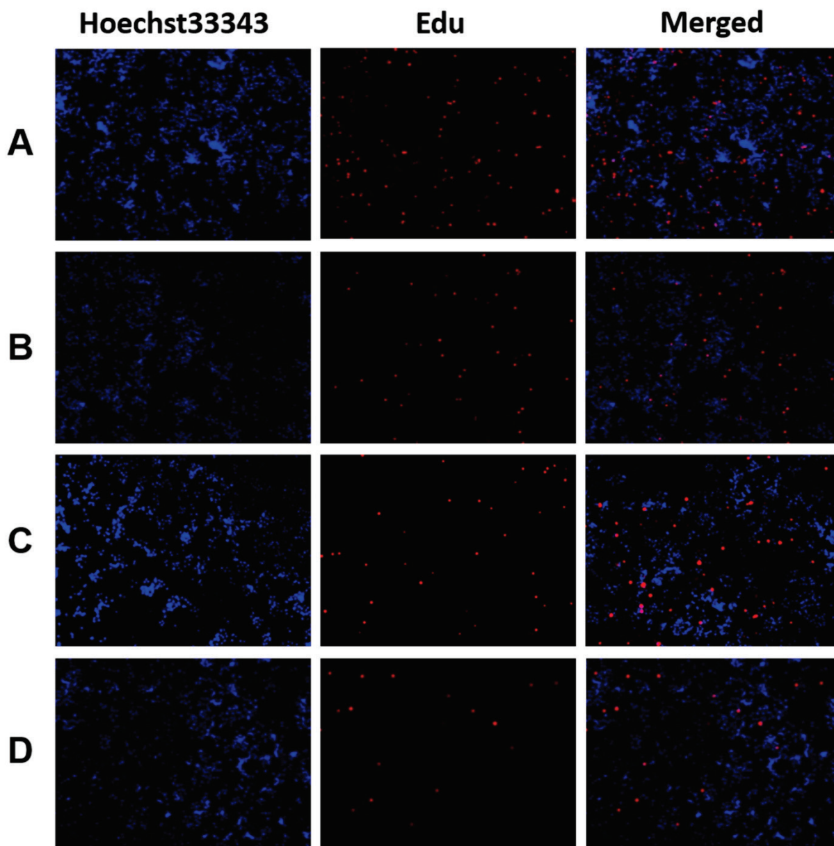
Fig. 2. EdU (5-ethynyl-2'-deoxyuridine) labels cells proliferating in primary chicken hepatocytes. (A) Control group. (B) Hepatocytes treated with 0.1 \mu\text{M} DHEA. (C) Hepatocytes treated with 1 \mu\text{M} DHEA. (D) Hepatocytes treated with 10 \mu\text{M} DHEA. The cells in each group were stained with DNA marker (Hoechst33342) and EdU, the merged images in the right column and the pink color in the merged image shows the proliferating cells.
