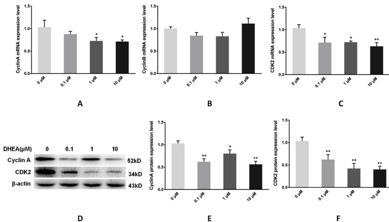
Fig. 4. Effect of DHEA on cell cycle related factors expression level in primary chicken hepatocytes. (A) Cyclin A mRNA expression level. (B) Cyclin B mRNA expression level. (C) CDK2 mRNA expression level. (D) Chicken hepatocytes were treated with 0, 0.1, 1 or 10 \mu\text{M} DHEA, and the protein were immunoblotted against cyclin A and CDK2. (E) Cyclin A protein expression abundance. (F) CDK2 protein expression abundance. Data are presented as means \pm SE from three individual experiments ( n=12 ). * P<0.05 , ** P<0.01 , DHEA treated group vs. control group.
