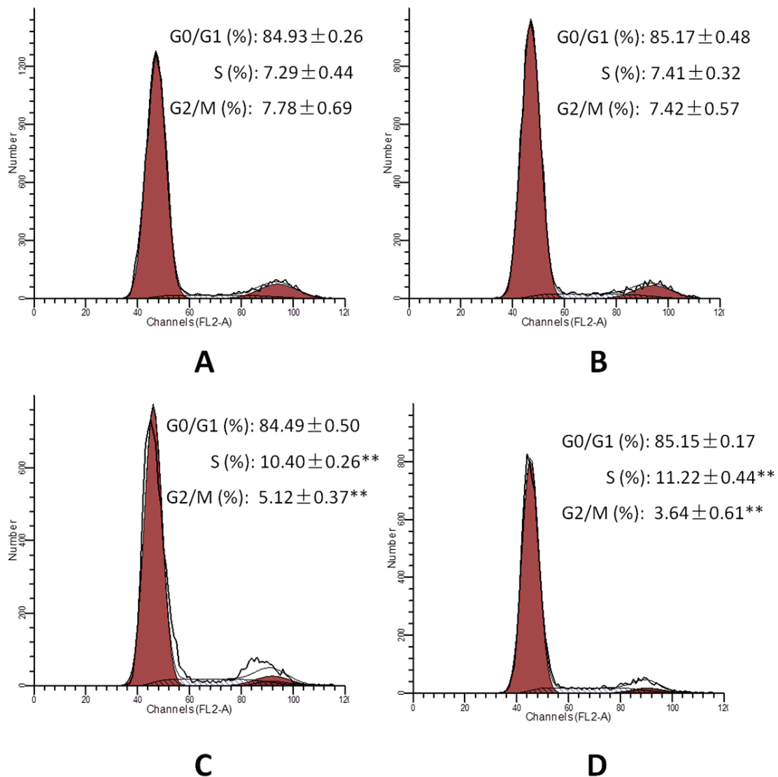
Fig. 3. Effect of DHEA on cell cycle in primary chicken hepatocytes. (A) Control group. (B) Hepatocytes treated with 0.1 μM DHEA. (C) Hepatocytes treated with 1 μM DHEA. (D) Hepatocytes treated with 10 μM DHEA. The cell cycle was evaluated using flow cytometric analysis, and cell cycle distribution was calculated from 10,000 cells with ModFit LTTM software using FACSCaliber. Data are presented as means ± SE from three individual experiments (n=12). ** P < 0.01 , DHEA treated group vs. control group.
