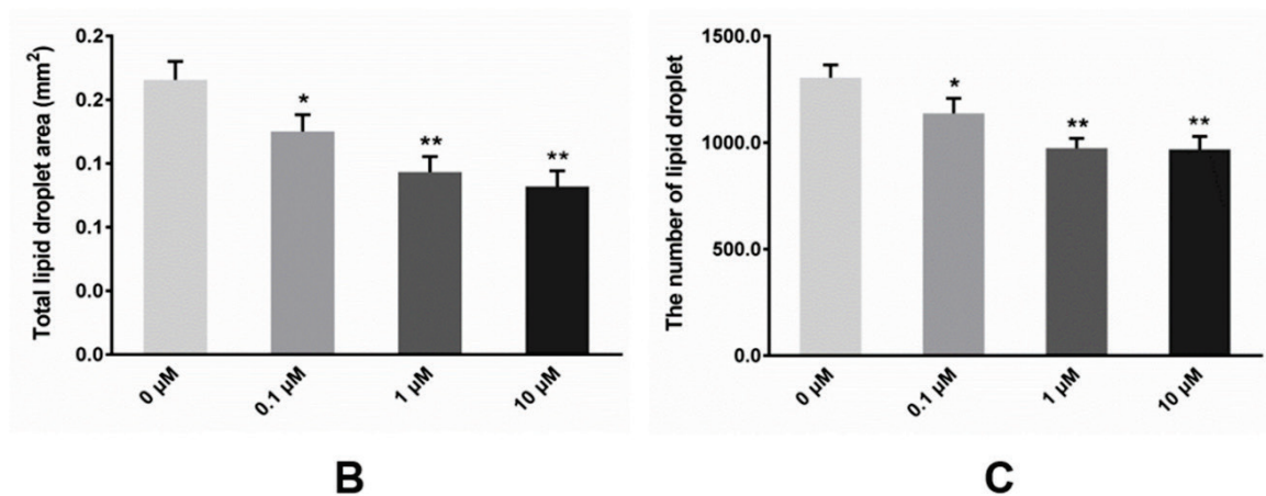
Fig. 1. Effect of DHEA on lipid droplets accumulation in primary chicken hepatocytes. (A) Representative photomicrographs of hepatocytes stained with Oil Red O, the red represents lipid droplet and blue represents the cell nucleus. (B) Total area of lipid droplets. (C) The number of lipid droplets. Data are presented as means \pm SE. * P < 0.05 , ** P < 0.01 , DHEA treated group vs. control group.
