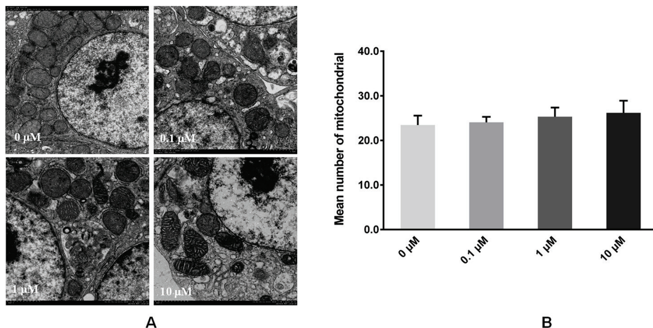
Fig. 5. Electron micrographs and the number of mitochondria in primary chicken hepatocytes treated with DHEA. (A) Electron micrographs. (B) The number of mitochondria. After incubation, cell samples were processed by standard techniques for transmission electron microscopy, and ultra-thin sections were observed with magnification \times 2,500 . Thirty photos were randomly selected from each treatment group, and fifteen independent cells in each photo were counted the number of mitochondria. The results are displayed as the average number of mitochondria per cell in all treatment groups and presented as means \pm SE.
