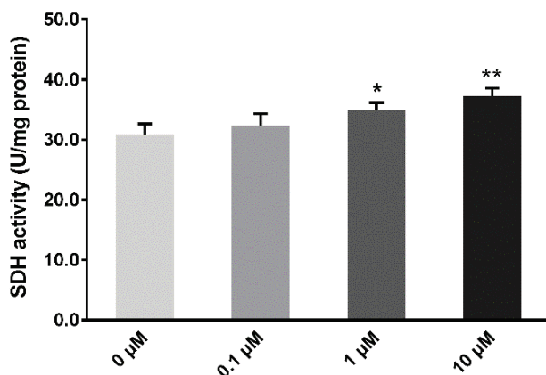
Fig. 7. Effect of DHEA on succinate dehydrogenase activity in primary chicken hepatocytes. The activity of succinate dehydrogenase (SDH) was normalized to the sample protein concentration as determined by a protein assay kit, and expressed as U/mg protein. Data are presented as means \pm SE from three individual experiments ( n=12 ). * P < 0.05 , ** P < 0.01 , DHEA treated group vs. control group.
