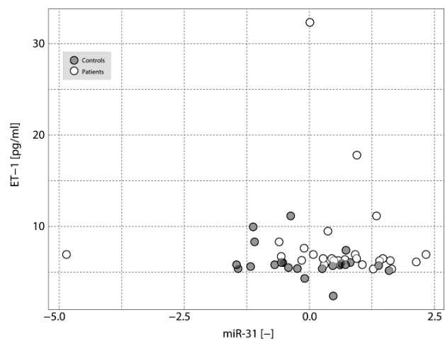
Fig. 1. The scatter plot depicts the serum levels of endothelin-1 (ET-1) and miR-31 in patients with psoriasis ( n=29 ) and control subjects ( n=22 ). Each point represents a single subject (open circles: patients, dark circles: controls). While there was no significant relationship between ET-1 and miR-31 in controls (Spearman's \rho = -0.13 , p = 0.556 ), for patients, we found a significant negative correlation between ET-1 and miR-31 (Spearman's \rho = -0.37 , p = 0.05 ).
