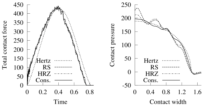
Fig. 3. Influence of mass lumping techniques on contact forces (left) and contact pressures (right) for IGA.
