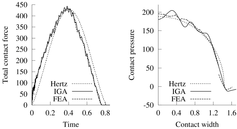
Fig. 2. Comparison of classic FEA and IGA solution of contact forces (left) and contact pressures (right) for HRZ mass lumping method.
