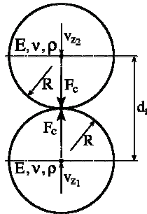
Fig. 1. Dynamic Hertz problem.
