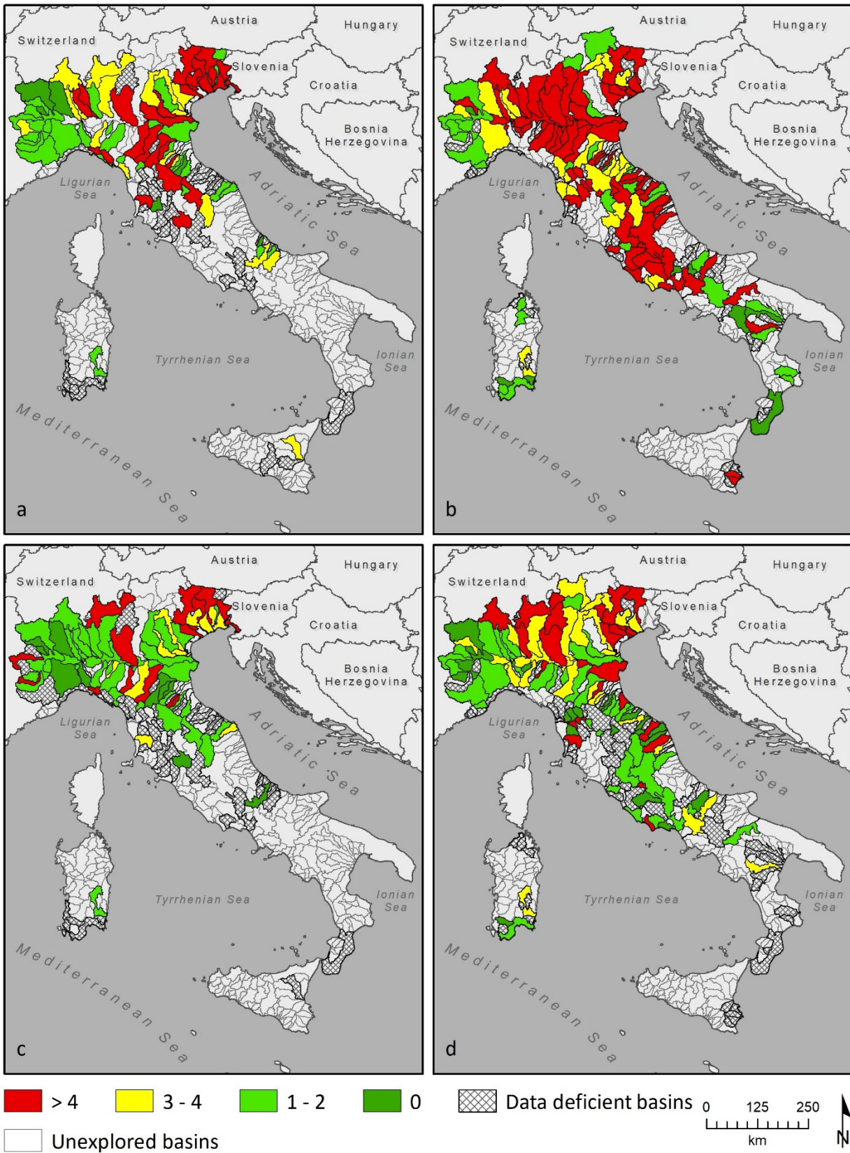
Fig. S4. Data completeness, i.e. difference between estimated and observed species richness: a) 1984-1999 overall; b) 2000-2014 overall; c) 1984-1999 native; d) 2000-2014 native).
