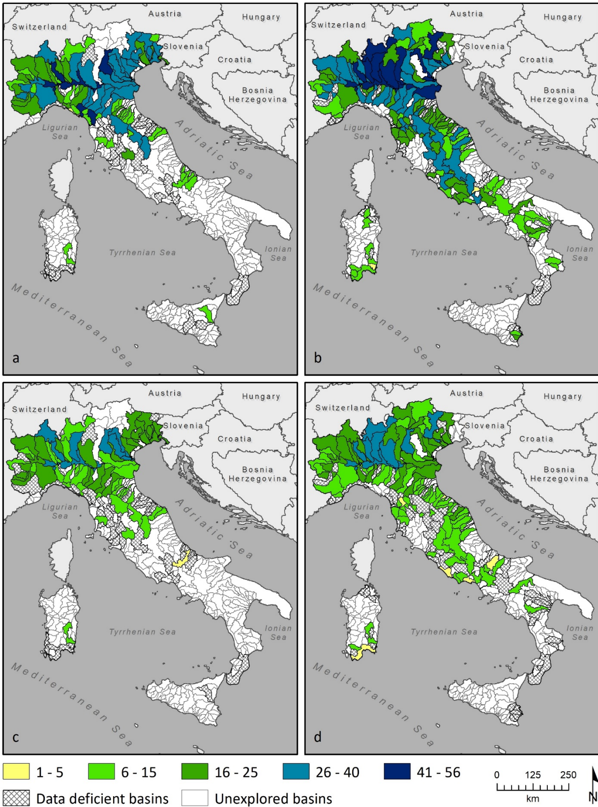
Fig. S3. Estimated species richness: a) 1984-1999 overall; b) 2000-2014 overall; c) 1984-1999 native; d) 2000-2014 native).
