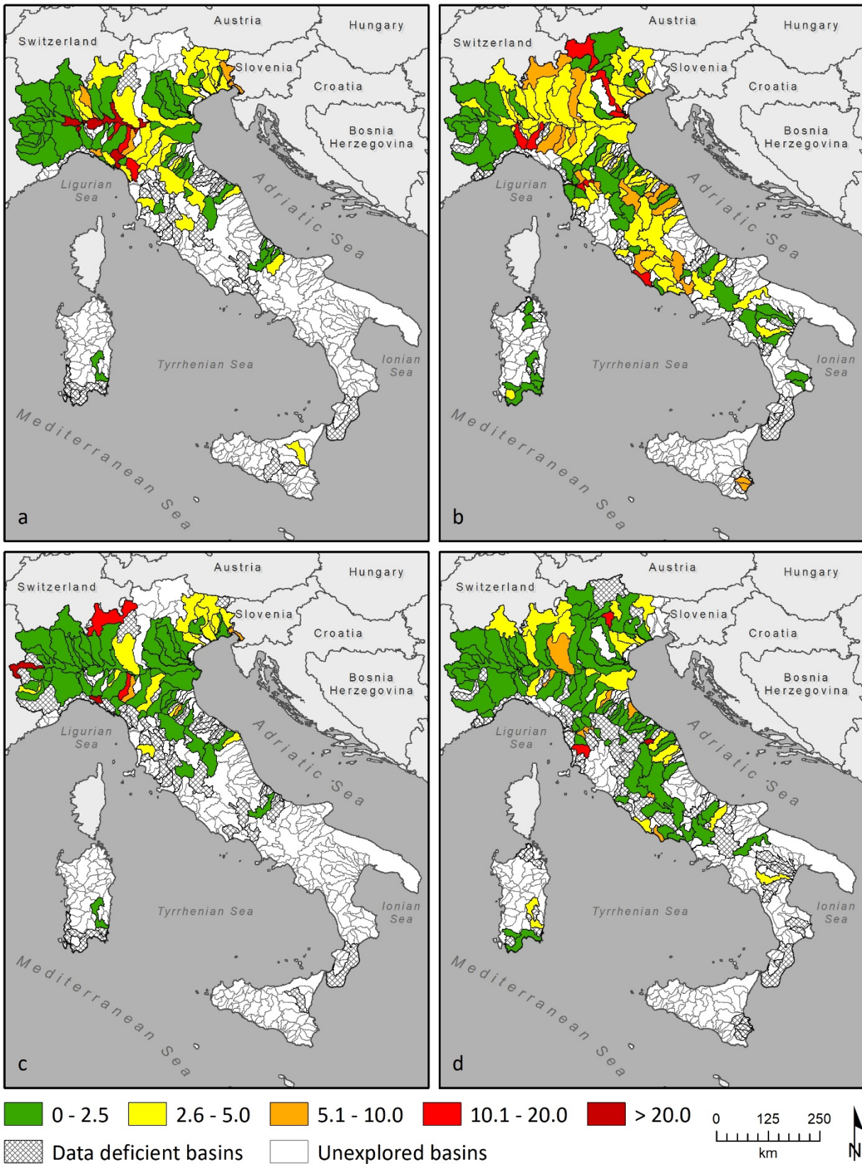
Fig. S5. Standard error of the species richness estimates: a) 1984-1999 overall; b) 2000-2014 overall; c) 1984-1999 native; d) 2000-2014 native).
