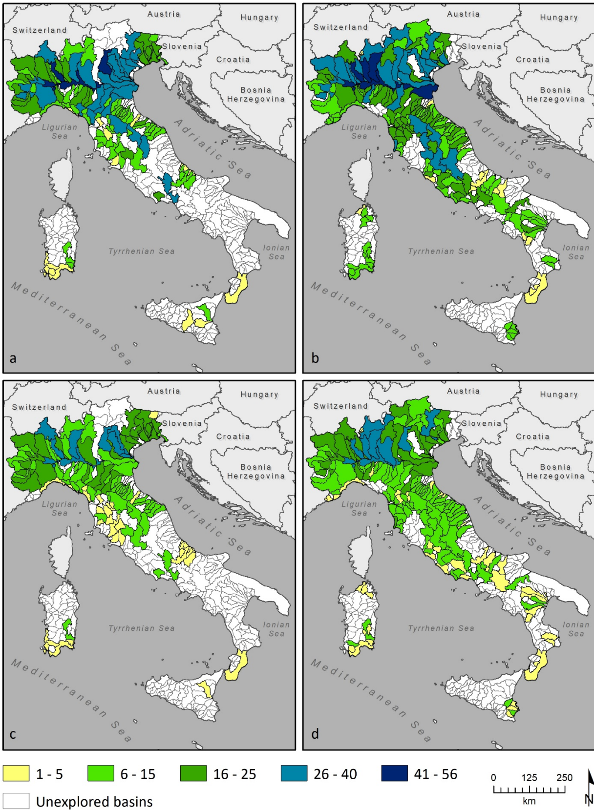
Fig. S2. Observed species richness: a) 1984-1999 overall; b) 2000-2014 overall; c) 1984-1999 native; d) 2000-2014 native).
