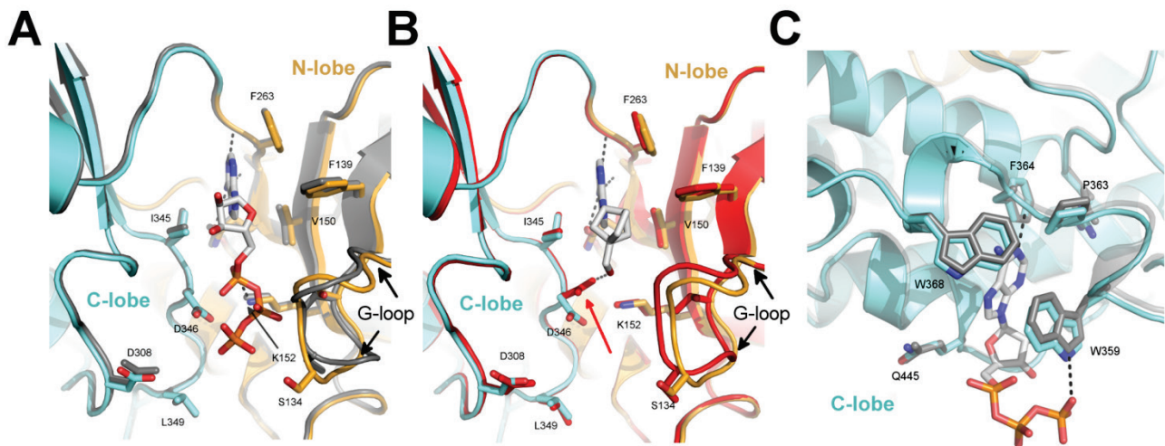
Fig. 2. Comparison of the ATP binding sites. A) The apo and ATP bound active site. C-lobe is colored in cyan, N-lobe in orange and T4 lysozyme in gray. The superimposed ATP bound kinase (pdb code 4PLA) is in gray except for the ATP that is colored according its elements. B) The apo and MD59 bound active sites. C-lobe is colored in cyan, N-lobe in orange and T4 lysozyme in gray. The superimposed ATP bound kinase (pdb code 4YC4) is in red except for the ATP that is colored according its elements. The red arrow points to the flexible D346 residue. C) The apo and ATP bound lateral pocket. C-lobe is colored in cyan. The superimposed ATP bound kinase (pdb code 4PLA) is in gray except for the ATP that is colored according its elements.
