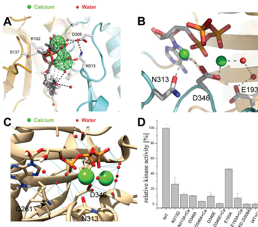
Fig. 3. Structural and functional analysis of PI4K II \alpha inhibition by calcium. A) The network of hydrogen bonds in the active site. C-lobe is colored in cyan, N-lobe in orange. The ATP is colored according to its elements. Calcium is shown as green spheres, water molecules as red spheres. The unbiased Fo-Fc map at 3 \sigma is shown for the calcium atoms. B) Detailed view of the active site. Colored as previous panel. C) The complex water network that holds the two calcium atoms in place. D) Mutagenesis analysis of the active site. The activity of each mutant was measured with and without 10 mM calcium ions and compared to the wt-enzyme.
