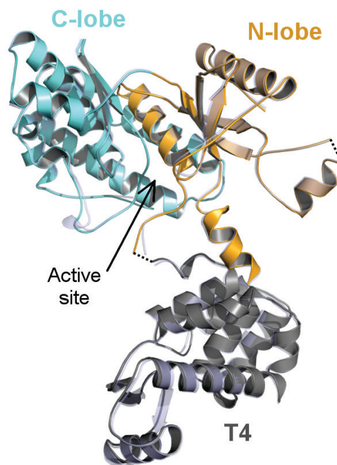
Fig. 1. The overall fold of PI4K II \alpha . The general fold is the same in the apo and liganded state. C-lobe is colored in cyan, N-lobe in orange and T4 lysozyme in gray. The superimposed liganded kinase (pdb code 4PLA) is colored in light blue and transparent.
