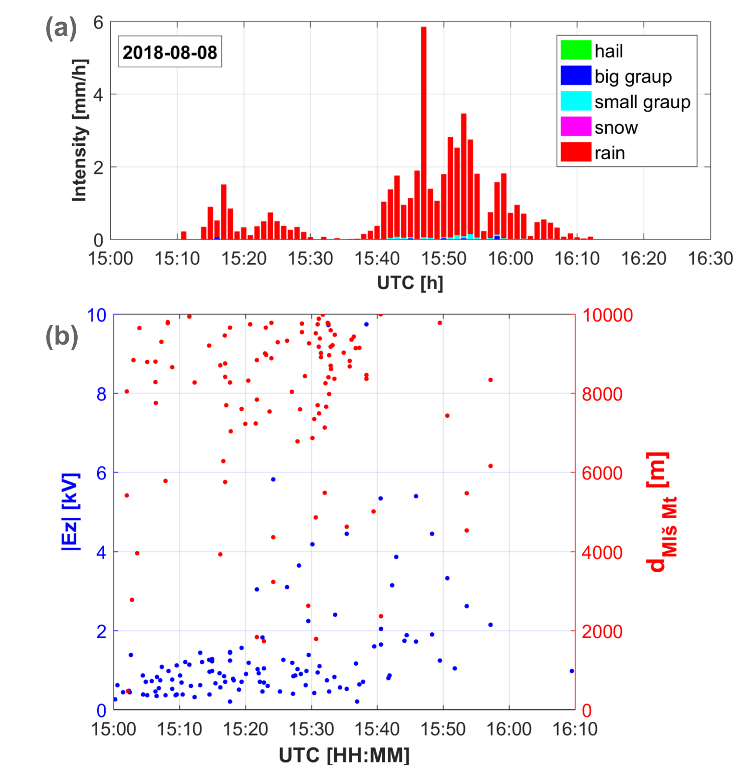
Fig. 4 Event on Aug 8, 2018: (a) Intensity of hydrometeors based on disdrometer data; (b) Changes in electric field based on data of electric field monitor and flashes recorded up to 10 km from the Milešovka Mt. by BLIDS.
