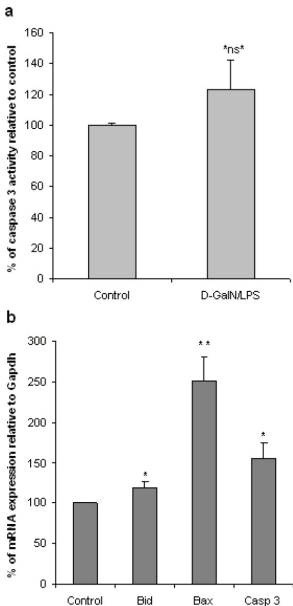
Fig. 4. Effect of lipopolysaccharide-induced hepatitis in D-galactosamine sensitized rats (D-GalN/LPS) on Caspase 3 activity (a) and on Bid, Bax and Casp 3 gene expressions relative to Gapdh as the endogenous control (b) 24 h after injection. Control: vehicle only; D-GalN/LPS: D-galactosamine 400 mg/kg with lipopolysaccharide 50 \mu g/kg; Values are mean \pm S.E.M., n=8; *ns* non-significant value compared to the negative control group (Control) p > 0.05 ; *,** value significant compared to Control p \leq 0.05^* , p \leq 0.01^{**} .
