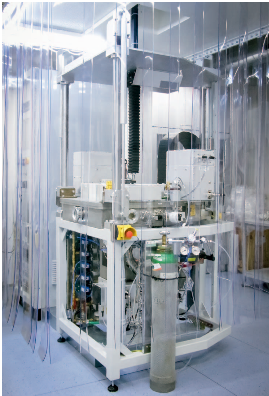
Computer controlled magnetron sputtering system Aurion
