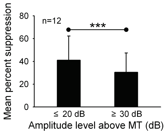
Fig. 3. Mean percent suppression of spikes in non-monotonic IC_{Rec} neurons during focal IC_{ES} ES. Bars show the mean percent suppression in spikes caused by focal IC_{ES} ES for two ranges of stimulus amplitude: \leq 20 dB above each neuron's MT and \geq 30 dB above each neuron's MT. n, the number of neurons; ***, P < 0.001 (paired t -test).
