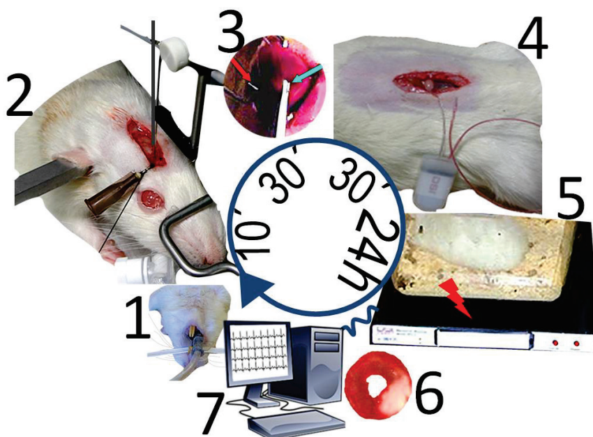
Fig. 1. The study-protocol included, (1) intubation (2) intracerebroventricular injections, (3) induction of myocardial infarction, (4) implantation of telemetry-recorders, (5) 24 h ECG-recording in conscious animals, (6) measurement of infarct-size, and (7) arrhythmia-analysis.
