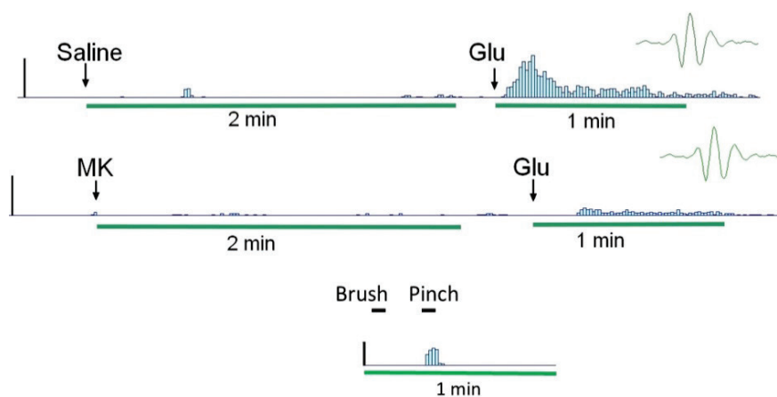
Fig. 3. Examples of the response of a single ON-like neuron in the periaqueductal gray (PAG) following microinjections of drugs into the right central nucleus of the amygdala (CeA). The uppermost row shows that saline failed to influence the discharge rate whereas 100 \mu g of glutamate induced a short-lasting increase in the discharge rate. The middle row shows that MK-801 at the dose of 2 \mu g failed to influence the discharge rate, while it prevented the glutamate-induced increase of the discharge rate. The lowermost row shows that prior to drug administrations, the PAG neuron was activated by noxious pinching of the tail but not by innocuous brushing. The insets show the shape of the action potential in the studied PAG neuron and the vertical calibration bars represent 50 Hz.
