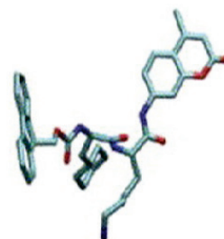
Fig. 3. Structure of galnon. A low molecular weight galanin receptor agonist galnon, 7-((9-fluorenylmethoxycarbonyl)cyclohexylalaninylsyl)amino-4-methylcoumarin (IUPAC name 9H-fluoren-9-ylmethyl N-[(2S)-1-[(2S)-6-amino-1-[(4-methyl-2-oxo-oxochromen-7-yl)amino]-1-oxohexan-2-yl]amino)-3-cyclohexyl-1-oxopropan-2-yl]carbamate) was discovered by application of a combinatorial library approach. Galnon possesses agonist properties in vitro and in vivo and strong anticonvulsant properties in vivo (Saar et al. 2002).
