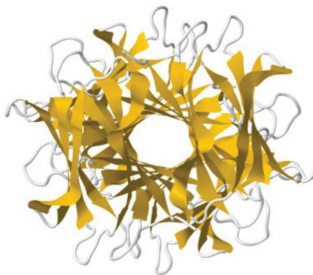
Fig. 1. Three dimensional structure of the galanin molecule.
