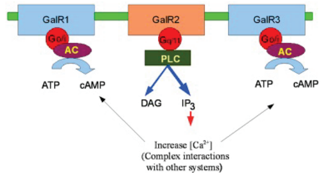
Fig. 2. The galanin receptors act through stimulation of different second messenger systems. The biological activity of GalR1 and GalR3 stimulation is linked to the activity of adenylate cyclase and cyclic AMP (cAMP) production and stimulation of GalR2 receptor to the phospholipase C (PLC) activity. Gal receptors affect various classes of intracellular G proteins and influence multiple signal transduction pathways. Based on several presentations Klenerová and Hynie (Klenerova 2013, Klenerova and Hynie 2013, Klenerova and Hynie 2015).
