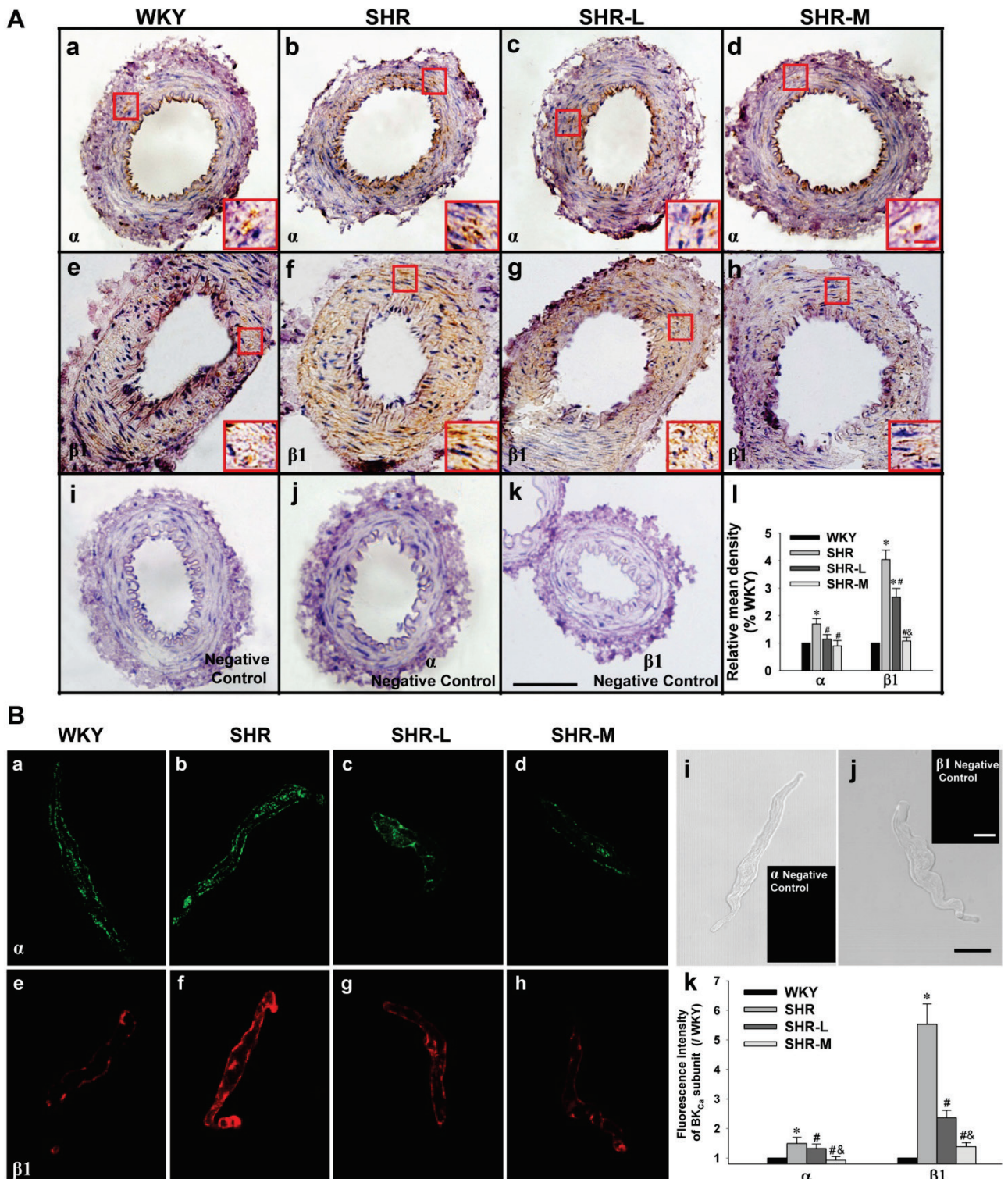
Fig. 4. BK Ca channel \alpha and \beta 1 subunits in MAs and VSMCs. A. Immunostaining of BK Ca subunits in MAs. ( a-h ) Representative positive immunostaining of \alpha subunit ( a-d ) and \beta 1 subunit ( e-h ) in WKY, SHR, SHR-L, and SHR-M. ( i ) Negative control performed by substituting primary antibody with a normal serum. ( j, k ) Immunoreactivity was abolished when the antibody was preabsorbed with excess peptide. The black scale bar represents 100 \mu m. The red scale bar in the insets represents 20 \mu m. ( l ) Summary of the relative mean integrated optical density (% WKY) in four groups. B. Fluorescent microphotographs of confocal microscopy images and quantitative analysis of BK Ca \alpha ( a-d ) and \beta 1 ( e-h ) subunits on arterial myocytes. ( i, j ) Bright field images of the VSMCs after staining. The inserts are representative images of VSMCs stained with \alpha or \beta 1 subunit antibody + blocking peptide. ( k ) The mean data illustrating the fluorescence intensity of the \alpha and \beta 1 subunit (WKY). Scale bar represents 20 \mu m. n=6 in each group. * P<0.05 , compared with WKY. # P<0.05 , compared with SHR. & P<0.05 , compared with SHR-L.
