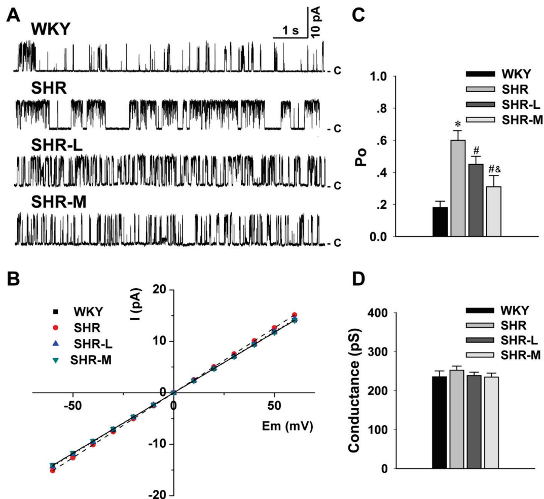
Fig. 3. Effects of exercise training on hypertension-associated alterations in BK_{Ca} channel activities and gating properties in MA myocytes. A. Single channel current recorded at a membrane voltage of +40 mV in WKY, SHR, SHR-L, and SHR-M ( [\text{Ca}^{2+}]_{\text{free}} = 1 \mu\text{M} ), respectively. B. I-V relationships of BK_{Ca} current. A linear fit revealed average single channel conductances ( G ) of 235.3 \pm 15.1 pS (WKY, n=12 cells/6 rats), 252.4 \pm 10.56 pS (SHR, n=15 cells/6 rats), 238.6 \pm 8.6 pS (SHR-L, n=13 cells/6 rats), and 234.5 \pm 10.3 pS, n=10 cells/6 rats, respectively. C, D. Summary of BK_{Ca} channel P_o ( C ) and conductance ( D ). * P < 0.05 , compared with WKY. # P < 0.05 , compared with SHR. & P < 0.05 , compared with SHR-L.
