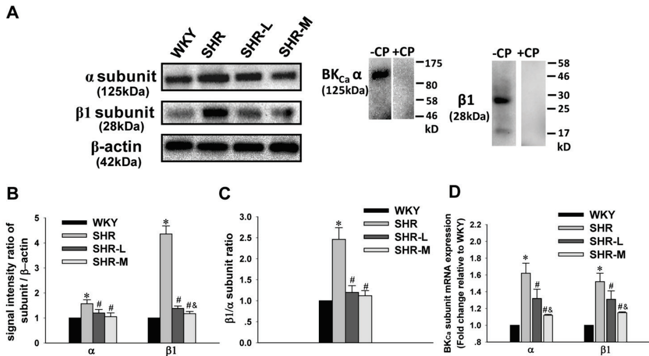
Fig. 5. Protein and mRNA in BK_{Ca} \alpha and \beta 1 subunits in mesenteric smooth muscle cells. A. Representative Western blot illustrating BK_{Ca} \alpha subunit, \beta 1 subunit, and \beta -actin. Specificity of the antibody was tested in mesenteric arterial smooth muscle lysate in Wistar rats. The immunoreactive band in the arterial tissue was abolished by preincubating with the corresponding control antigen, indicating specificity of the antibody for its intended epitope. B, C. Mean values of BK_{Ca} \alpha subunit and \beta 1 subunit proteins ( B ), and the \beta 1/\alpha ratio ( C ). D. Mean quantitative PCR data for BK_{Ca} \alpha and \beta 1 subunit mRNA in MAs normalized to \beta -actin and then to age-matched WKY controls. n=6 in each group. * P<0.01 , compared with WKY; # P<0.01 , compared with SHR; & P<0.01 , compared with SHR-L.
