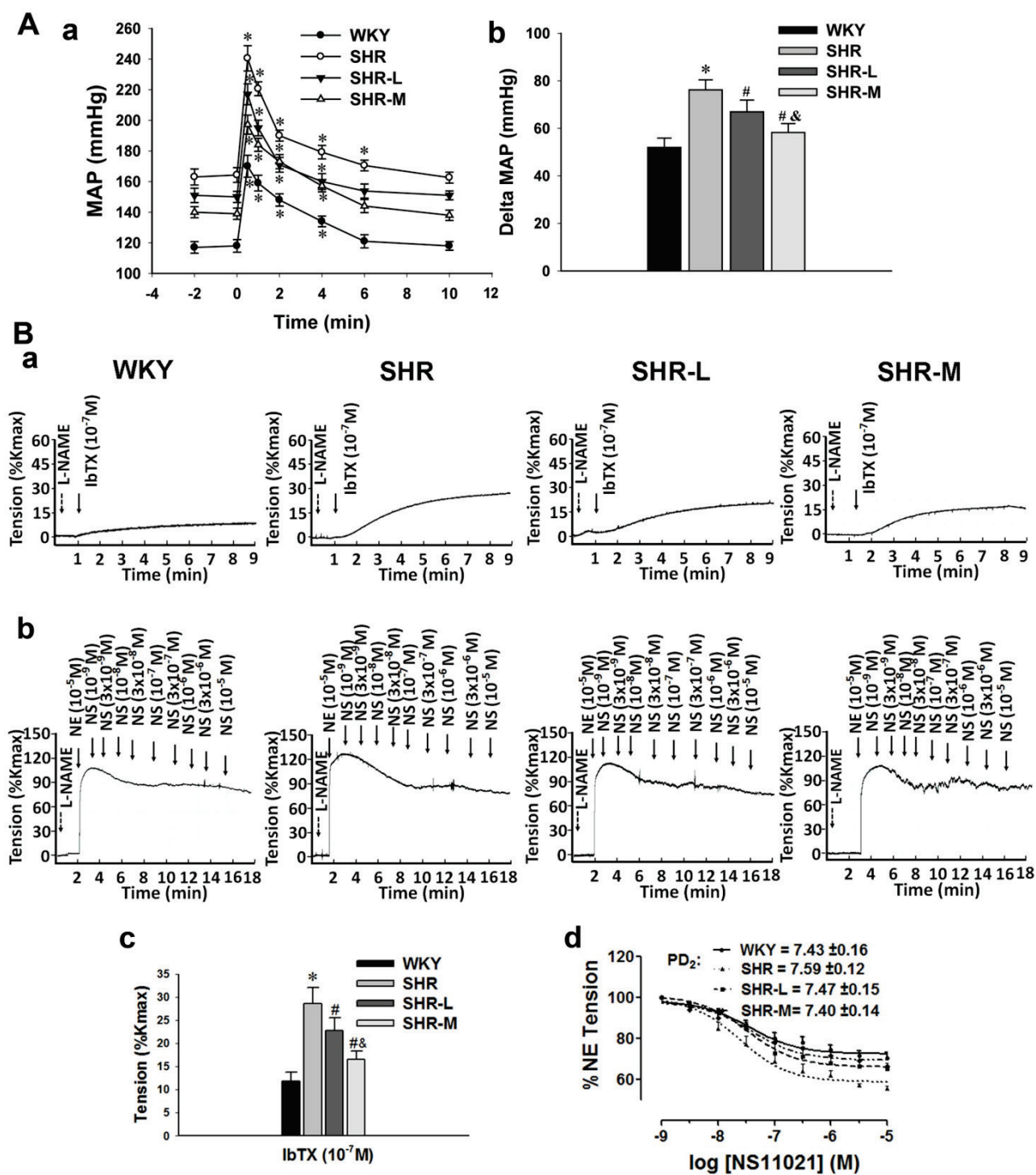
Fig. 1. Effect of exercise on NE-induced cardiovascular responses and vascular tension in MAs. A. Effect of exercise on NE-induced cardiovascular responses. (a) NE-induced MAP response; *P < 0.05 , compared with the baseline level. (b) The maximal change in MAP ( \Delta MAP) after injection of NE. NE, norepinephrine, 18 \mu g/kg. B. Effects of a BK Ca channel inhibitor and activator on vascular tension in MAs. (a) Typical experimental tracings showing effect of the BK Ca blocker, IbTX (100 nM), on resting tension. (b) Effect of the BK Ca channel activator, NS11021 ( 10^{-9} to 10^{-5} M), on NE-induced vessel contraction. In each experiment, the arteries were pre-incubated with the non-selective NOS inhibitor, L-NAME (100 \mu M), for 20 min (dotted arrows). (c) Statistical diagram of IbTX effects on NE-induced vessel contraction. (d) Concentration-response curves of NS11021 effects on NE-induced contraction. NS, NS 11021. *P < 0.05 , compared with WKY; \#P < 0.05 , compared with SHR; \&P < 0.05 , compared with SHR-L. n = 6 in each group.
