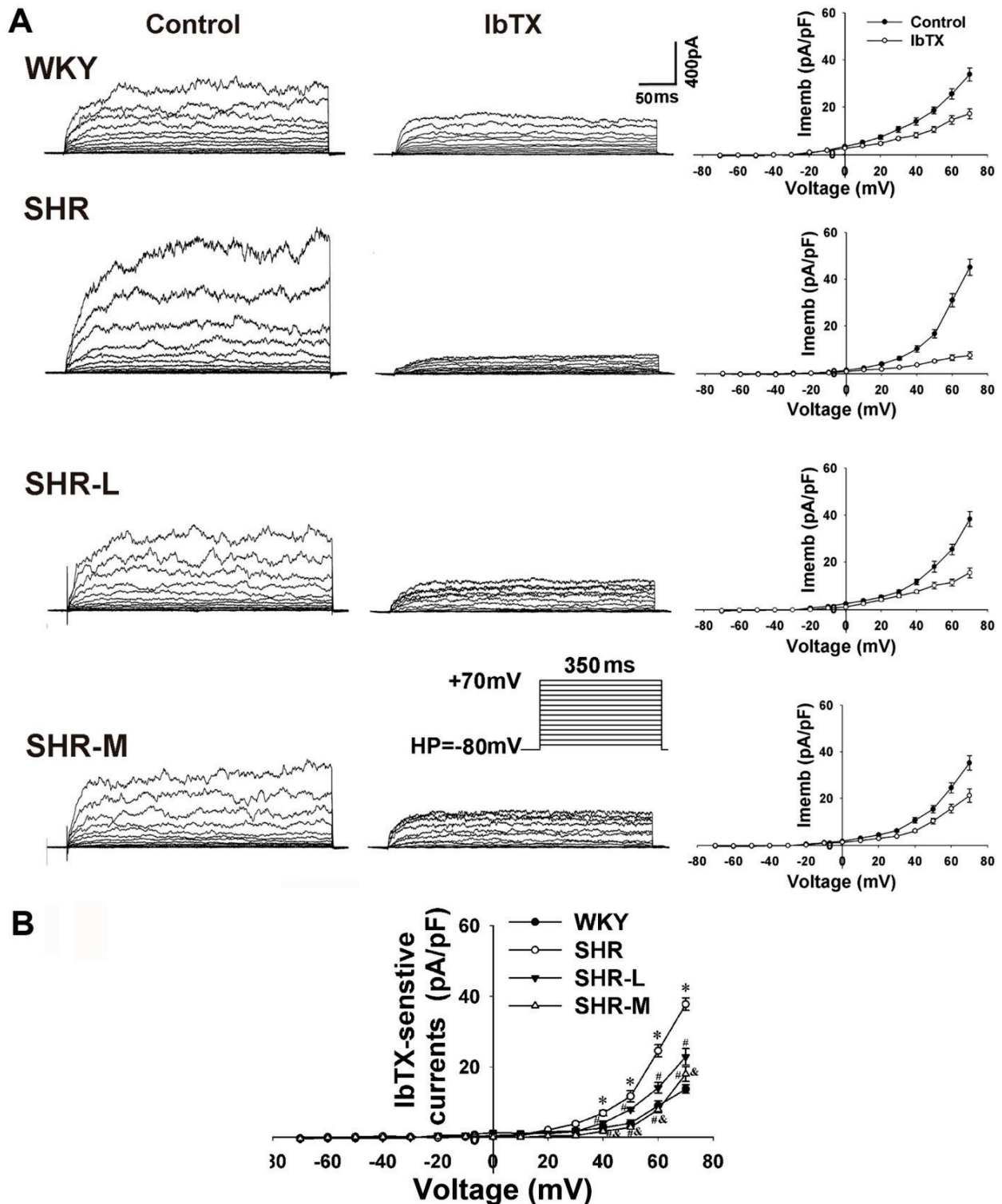
Fig. 2. Whole-cell K + currents in MA myocytes from WKY, SHR, SHR-L, and SHR-M. A. Typical recordings of whole-cell K + currents measured during depolarizing voltage steps in the absence (left panel) or presence of IbTX (100 nM, middle panel); the mean current density versus voltage plot (right panel) in the absence (closed circles) or presence (open circles) of IbTX. B. I-V relationships of BK Ca current density in VSMCs from four groups. SHR, n =18 cells from 6 rats; WKY, n =18 cells from 6 rats; SHR-L, n =14 cells from 6 rats; SHR-M, n =19 cells from 6 rats. * P <0.05, compared with WKY. # P <0.05, compared with SHR. & P <0.05, compared with SHR-L.
