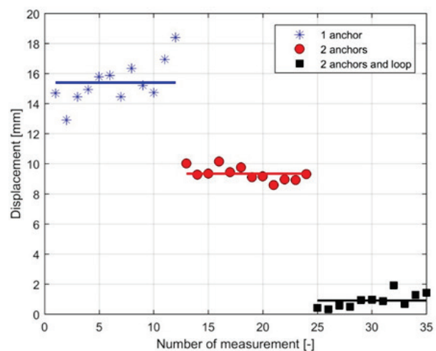
Fig. 7. Displacement of electrode for different anchoring wires.
