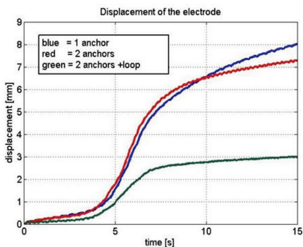
Fig. 6. Total displacement of the end of electrode.
