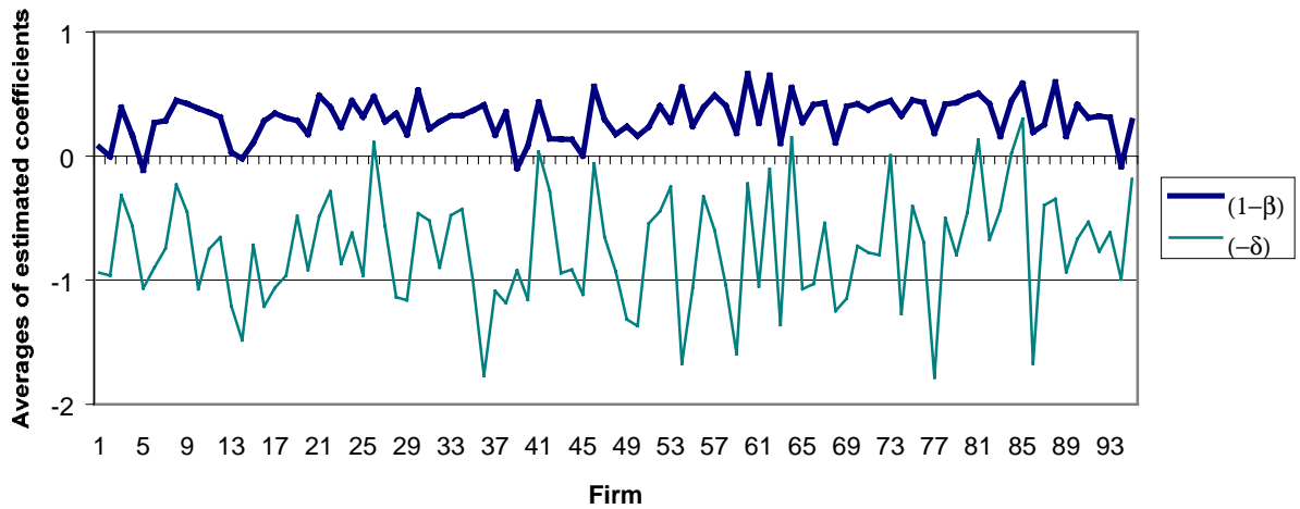
Figure 3. Time averages of the 90-day “rolling sample” estimates of (1-\beta) and (-\delta) for individual firms
