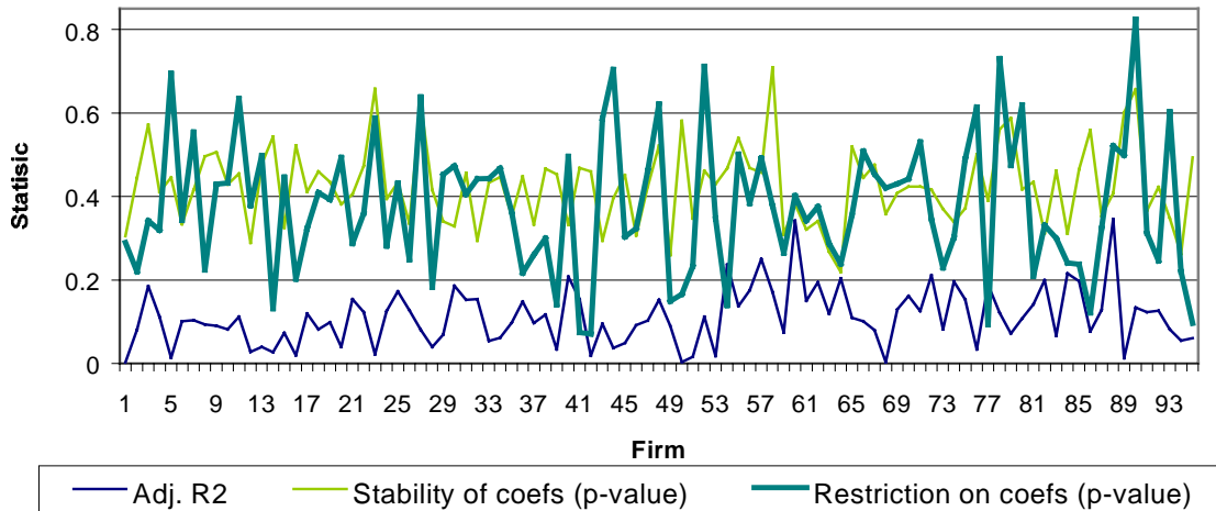
Figure 5. Time averages of the 90-day “rolling sample” specification statistics for individual firms
