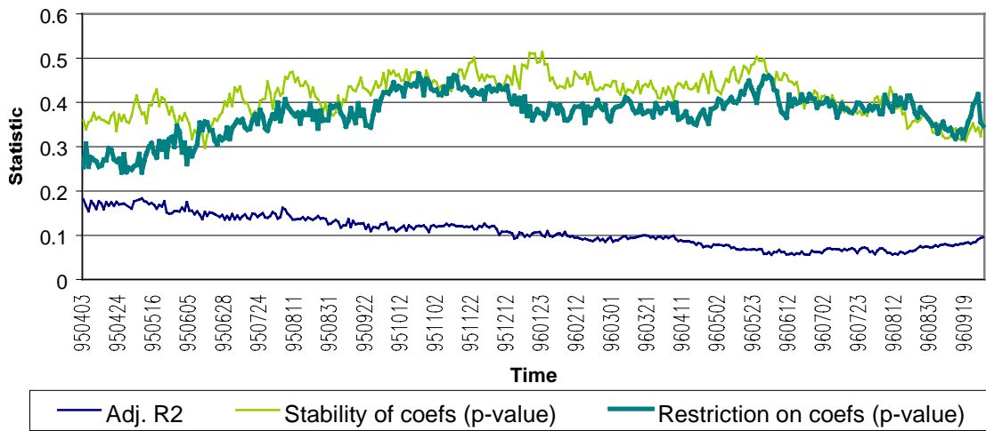
Figure 6. Cross-firm averages of the 90-day “rolling sample” specification statistics for different dates
