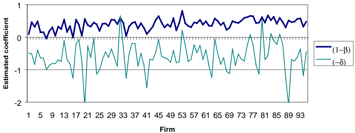
Figure 3. Time averages of the 90-day “rolling sample” estimates of (1-\beta) and (-\delta) for individual firms
