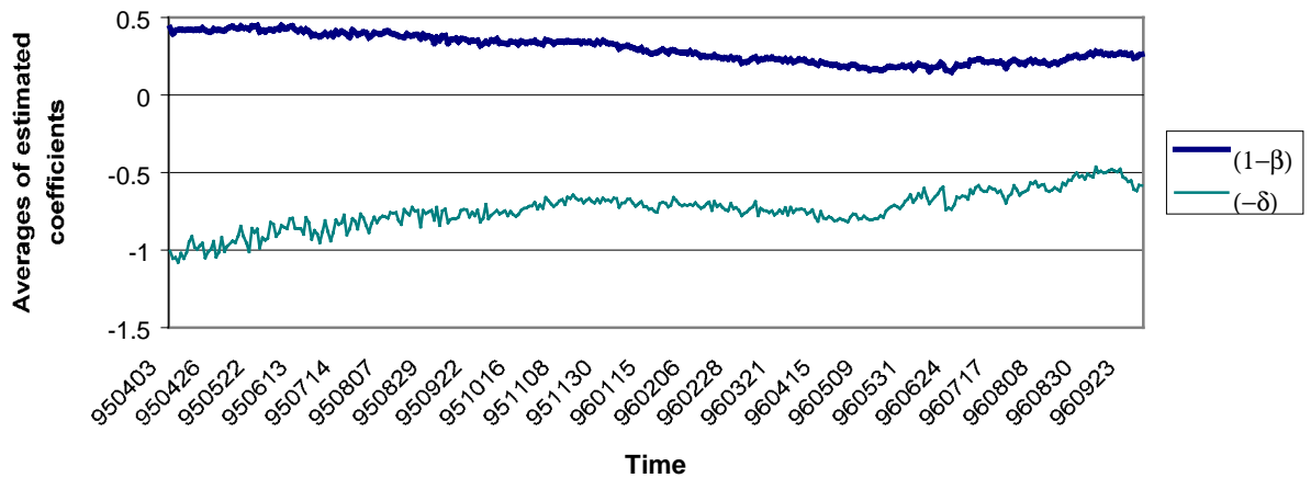
Figure 4. Cross-firm averages of the 90-day “rolling sample” estimates of (1-\beta) and (-\delta) for different dates
