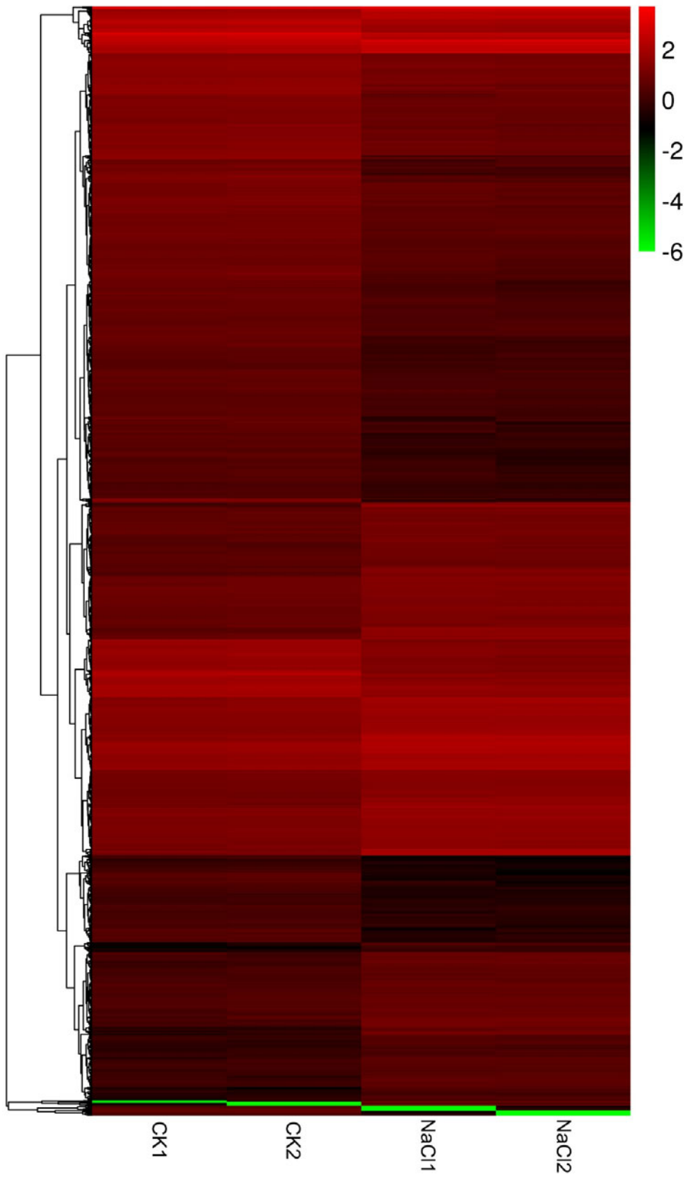
Fig. 4S. The expression patterns of differentially expressed genes compared by cluster analysis.
