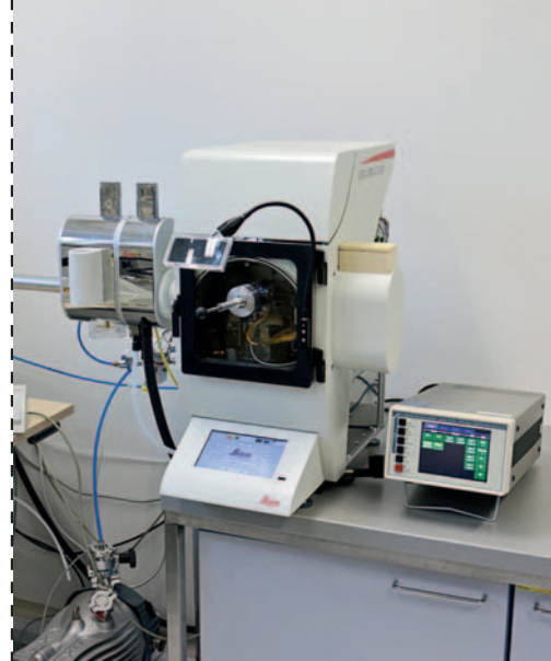
Equipment for cryo-SEM sample preparation
