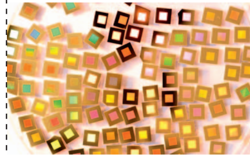
Specimens for Raman spectroscopy — etched silicon with Au nano-islands
