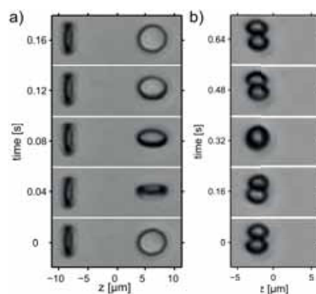
An example of simultaneous trapping and rotation of disc-like objects in counter-propagating laser beams with circular polarizations.
