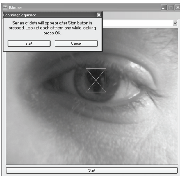
Fig. 1. Eye pupil tracking. The centre of the circumscribed rectangle is considered as the pupil's coordinates. The figure is a screenshot of the application before the calibration procedure.
