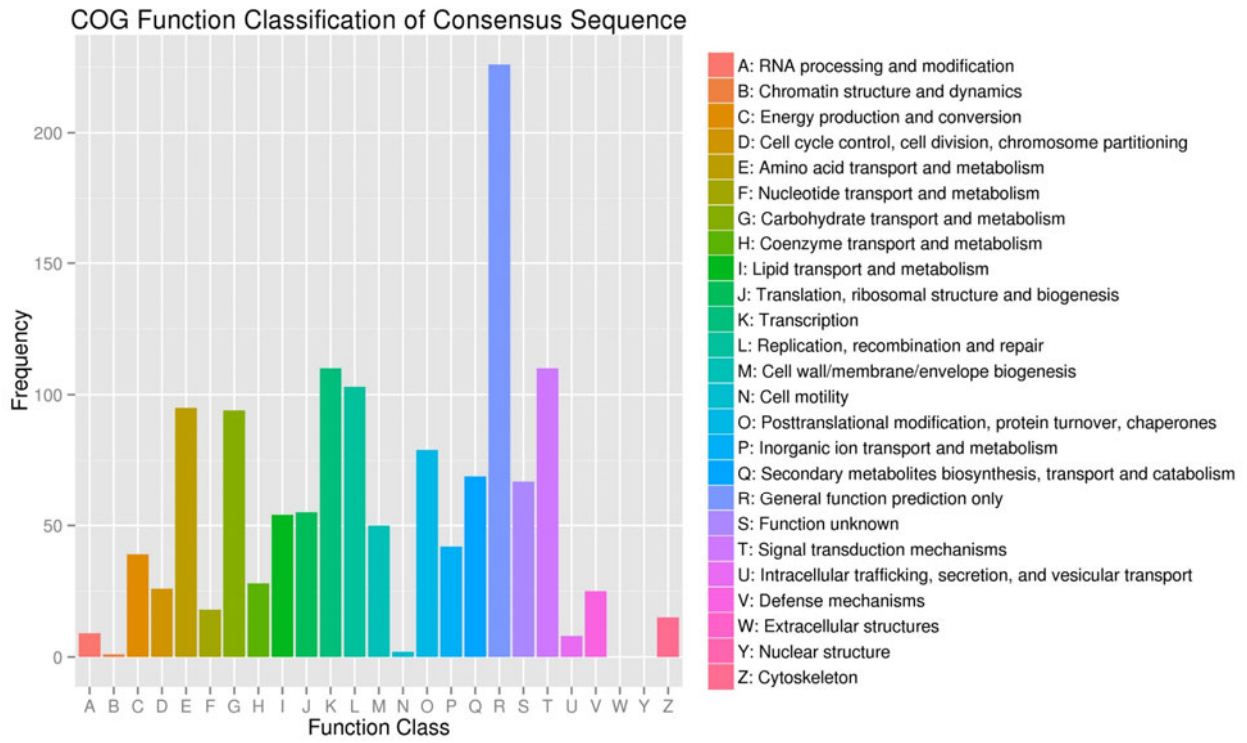
Fig. 2S. Functional annotation of assembled sequences based on clusters of orthologous groups (COG) categorization.
