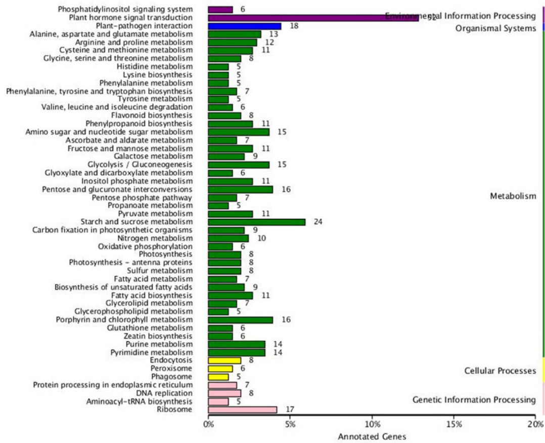
Fig. 3S. Functional annotation of assembled sequences based on Kyoto encyclopedia of genes and genomes (KEGG) categorization.
