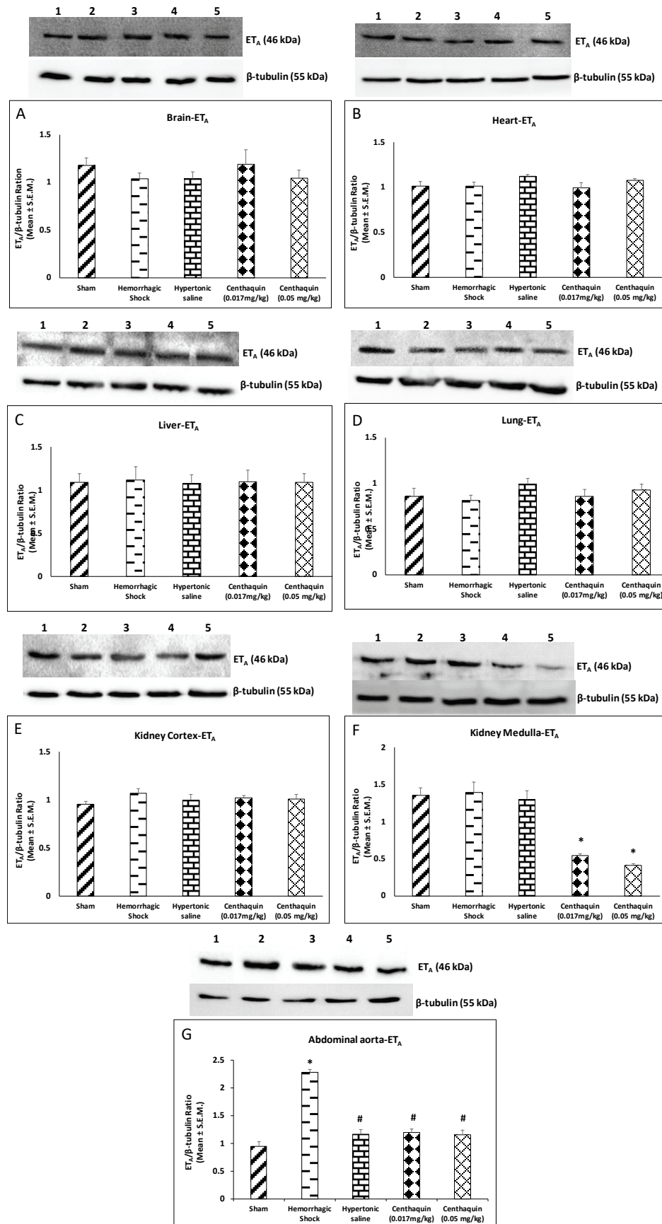
Fig. 2. Effect of hemorrhage on the expression of ET A receptors in sham and hemorrhaged rats. Hemorrhaged rats were resuscitated with hypertonic saline or centhaquin. Lane 1 – Sham, Lane 2 – Hemorrhagic shock, Lane 3 – Hypertonic saline (vehicle), Lane 4 – Vehicle + centhaquin (0.017 mg/kg), Lane 5 – Vehicle + centhaquin (0.05mg/kg). The values are expressed as mean ± SEM. (n=4). *p<0.05 compared to sham, #p<0.05 compared to hemorrhage or hypertonic saline.
