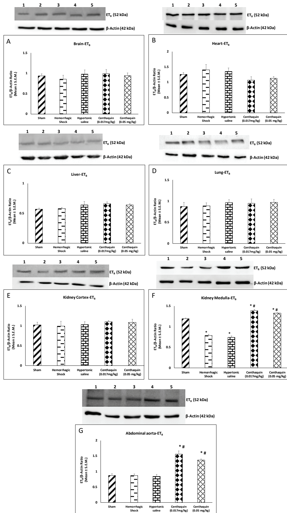
Fig. 3. Effect of hemorrhage on the expression of ET B receptors in sham and hemorrhaged rats. Hemorrhaged rats were resuscitated with hypertonic saline or centhaquin. Lane 1 – Sham, Lane 2 – Hemorrhagic shock, Lane 3 – Hypertonic saline (vehicle), Lane 4 – Vehicle + centhaquin (0.017 mg/kg), Lane 5 – Vehicle + centhaquin (0.05 mg/kg). The values are expressed as mean ± SEM. (n=4). *p<0.05 compared to sham, #p<0.05 compared to hemorrhage or hypertonic saline.
