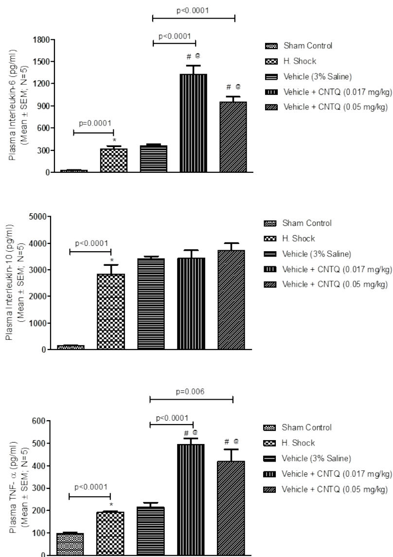
Fig. 4. Effect of hemorrhage on plasma TNF- \alpha , IL-6 and IL-10 in sham and hemorrhaged rats. Hemorrhaged rats were resuscitated with hypertonic saline or centhaquin. The values are expressed as mean \pm SEM. (n=5). *p<0.05 compared to sham, #p<0.05 compared to hemorrhage, @p<0.05 compared to hypertonic saline.
