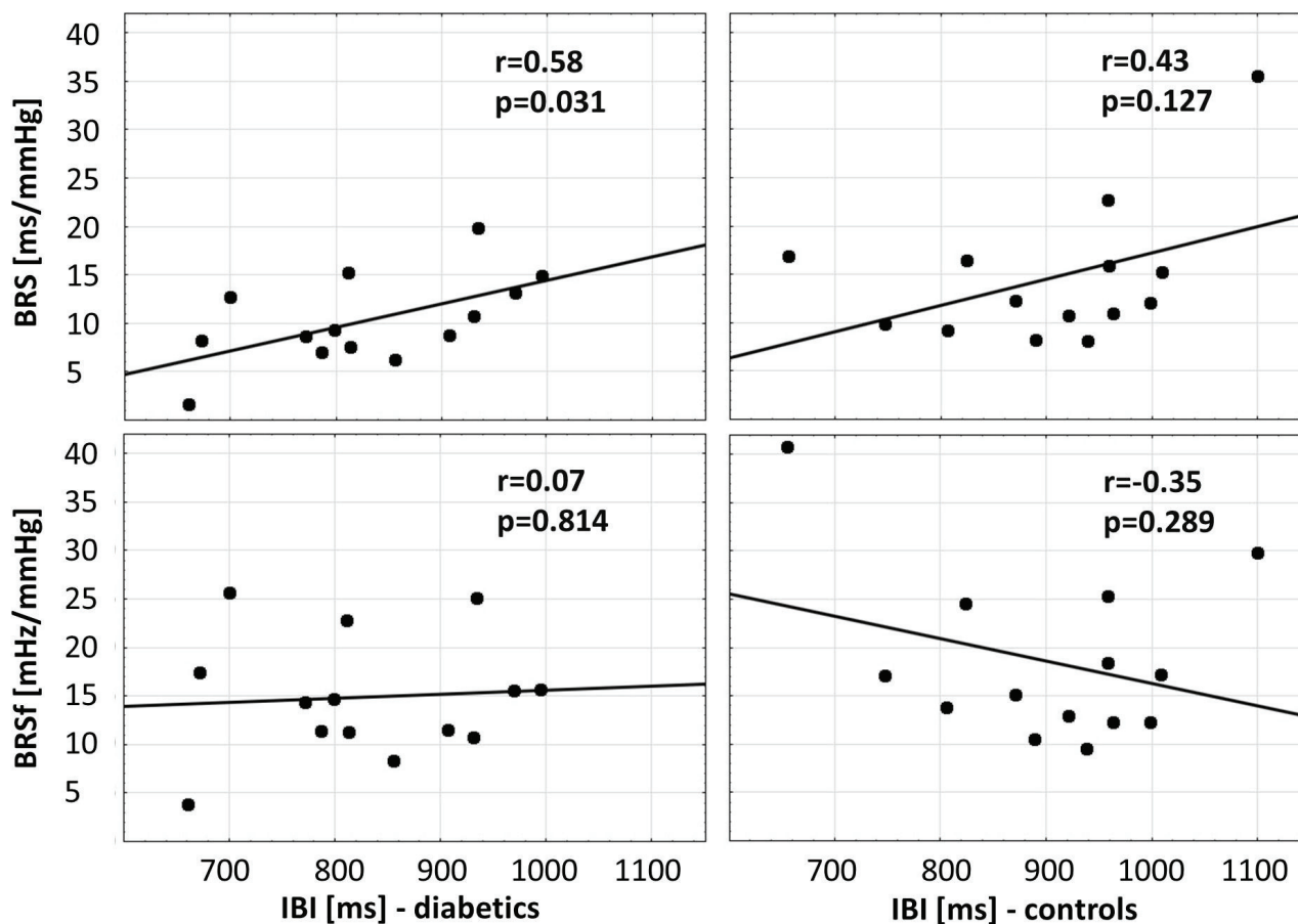
Fig. 3. Dependence of BRS and BRSf on inter-beat interval (IBI) in diabetics and controls.
