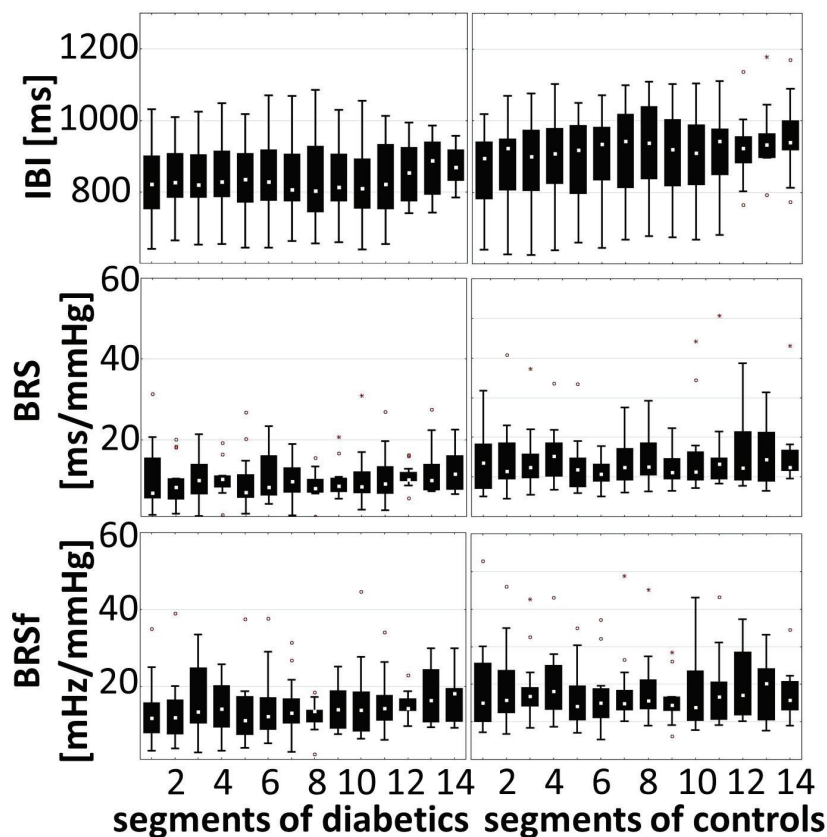
Fig. 2. Fluctuation of inter-beat intervals (IBI) and baroreflex sensitivity indices (BRS and BRSf) measured in controls and diabetics in 14 segments lasting 3 min within forty-two minutes. The box plots illustrate medians (white points), interquartile ranges and outliers (black points) of values in both groups in each segment.
