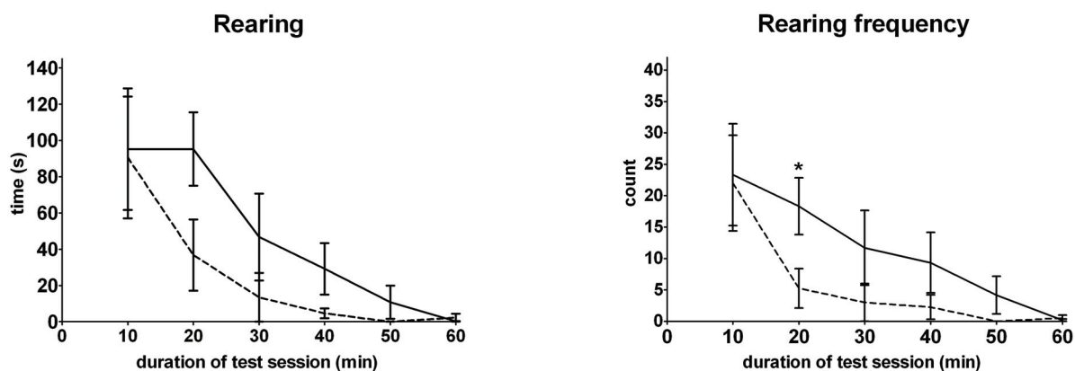
Fig. 4. Delayed NIC-induced effects on vertical and horizontal activity. Whole one hour session divided into six 10-minutes intervals. Solid lines represent NIC treated rats, dashed lines saline treated rats. * Results significant at p < 0.05 , ** results significant at p < 0.01 . Error bars were calculated as \pm SEM.
