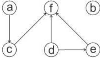
Figure 6: Elimination dag G^\circ(L)
