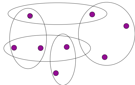
Figure 2: An example of a hypergraph
