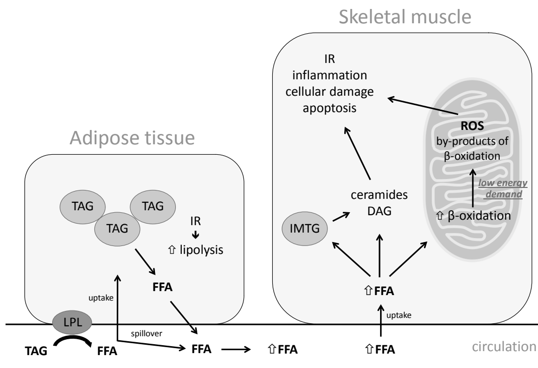
Fig. 1. A schematic view of obesity-associated, fatty acid-induced insulin resistance and metabolic dysfunction in skeletal muscle. An increased release of free fatty acids (FFA) from dysfunctional adipose tissue and a reduction in postprandial plasma triacylglycerols (TAG)/FFA clearance lead to higher circulating FFA levels/fluxes and higher uptake to skeletal muscle. FFA accumulated in skeletal muscle can be incorporated into intramyocellular TAG (IMTG) or oxidized in mitochondria. Excess FFA can then be converted to active lipid metabolites, such as ceramide and diacylglycerol (DAG). Oversupply of FFA drives an adaptive increase in mitochondrial \beta -oxidation, which, without an increase in energy demand, leads to incomplete fatty acid oxidation, increased redox pressure on the electron transport chain (ETC) and increased production of reactive oxygen species (ROS), with ensuing oxidative stress, development of insulin resistance (IR) and cellular damage.
