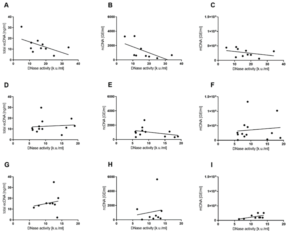
Fig. 2. Correlation of DNase activity with total ecDNA, ncDNA and mtDNA. No statistically significant correlations were found in any of the experimental groups. In females, no correlation of DNase with (A) ecDNA, (B) ncDNA and (C) mtDNA was observed. In control males, no correlation of DNase with (D) ecDNA (F), mtDNA and (E) ncDNA was observed. Similarly, in castrated males, no significant correlation of DNase activity with (G) ecDNA, (H) ncDNA and (I) mtDNA was found.
