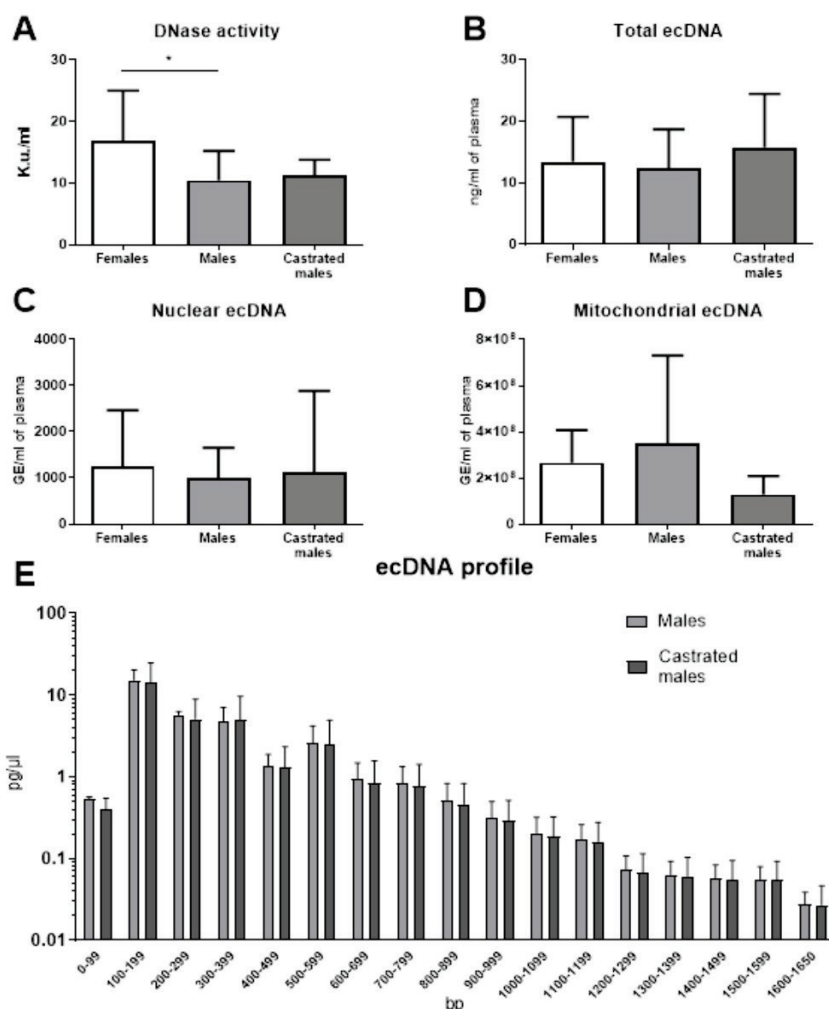
Fig. 1. DNase activity and ecDNA concentration in female, male and castrated male rats. (A) Significant differences in DNase activity were found between males and females but not between control males and castrated males. (B) No differences were observed between groups in concentration of total ecDNA. Similarly, no difference was found in concentration of (C) ncDNA and (D) mtDNA between groups. (E) Analysis of ecDNA profile of the distribution of DNA fragment lengths. No difference was observed in the length distribution of DNA fragments between males and castrated males. The results are shown as mean + standard deviation.
