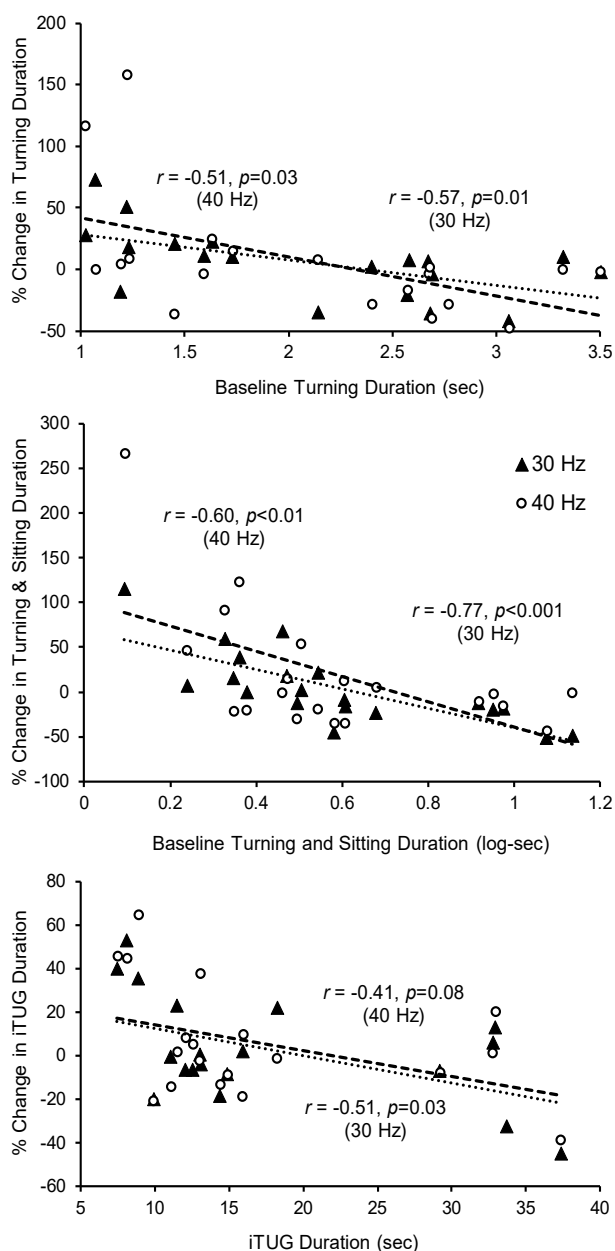
Fig. 2. Correlations between changes in instrumented Timed-Up-and-Go (iTUG) performance due to vibration and baseline iTUG performance.
