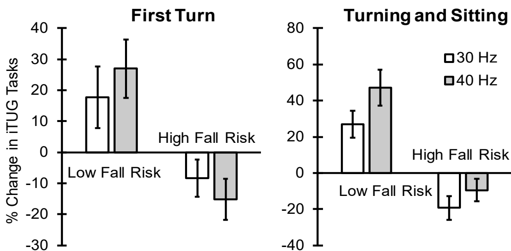
Fig. 1. Changes in instrumented Timed-Up-and-Go (iTUG) performance comparing vibration versus no-vibration trials.
