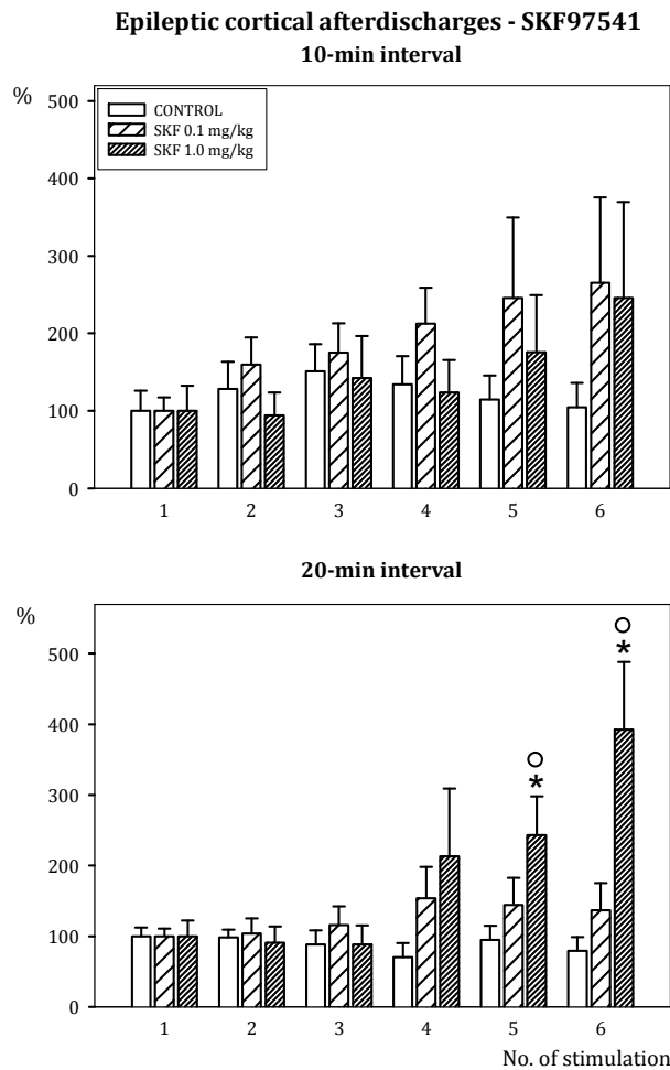
Fig. 2. Relative duration of six successive cortical ADs (mean + SEM). Upper graph – stimulation with 10-min intervals, lower graph – stimulation with 20-min intervals. Duration of the first AD in each dose group was taken as 100 %. Individual columns – see inset. Asterisks denote significant difference in comparison with appropriate first AD, circles – in comparison with corresponding control AD.
