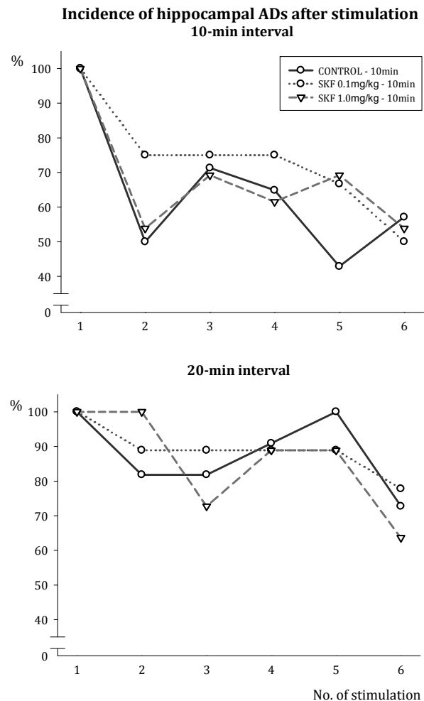
Fig. 4. Upper graph: Incidence of elicited hippocampal afterdischarges after each stimulation – incidence of stimulation with 10-min intervals. Details – see inset. Lower graph: Incidence of elicited hippocampal afterdischarges after each stimulation – incidence of stimulation with 20-min intervals. Details – see inset.
