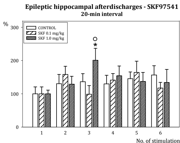
Fig. 3. Relative duration of six successive hippocampal ADs elicited with 20-min intervals (mean + SEM). Details as in Figure 2.
