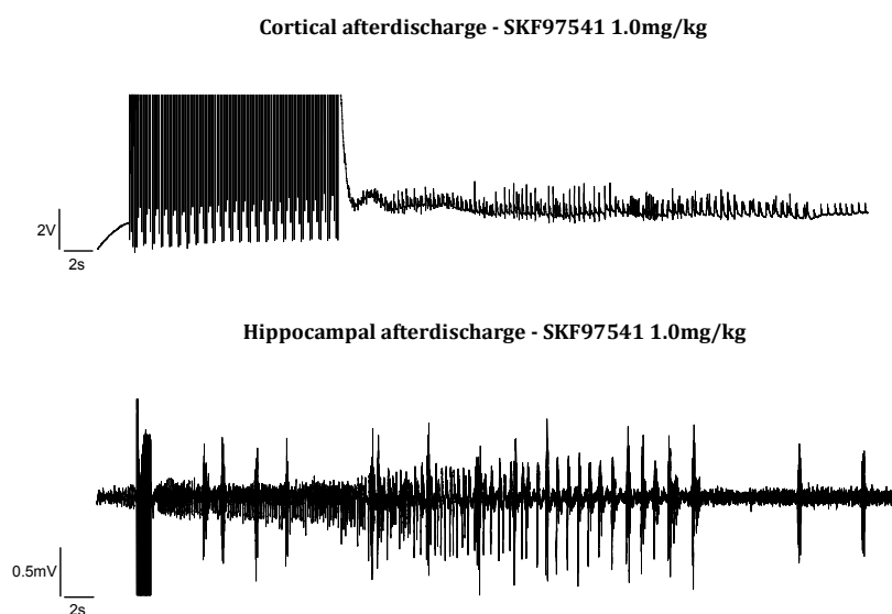
Fig. 1. EEG recording of cortical afterdischarge (AD) from sensorimotor area opposite to stimulation electrodes ( upper part ). EEG recording of hippocampal AD from dorsal hippocampus opposite to stimulation site ( lower part ). Activity was recorded in reference connection, amplitude and time mark – see inset.
