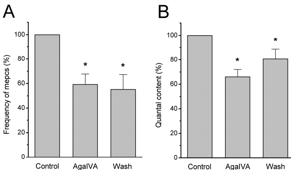
Fig. 4. Effects of \omega -agatoxin IVA on spontaneous and evoked quantal release of mediator at frog neuromuscular junction. Decrease in mEPSC frequency ( panel A ) and quantal content ( panel B ) expressed as a percentage of control values, set as 100 %. Asterisks (*) indicate a statistically significant difference ( p < 0.05 ) from the control value.
