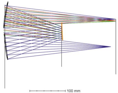
Optical design simulation of hyperspectral camera.
