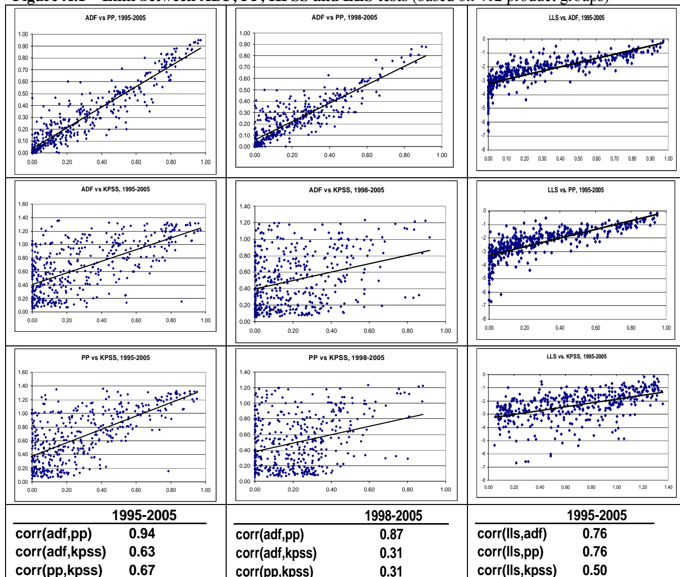
Figure A.1 – Link between ADF, PP, KPSS and LLS tests (based on 412 product groups)
