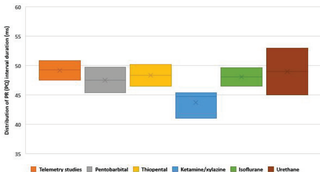
Fig. 2. Distribution of ranges of PR(PQ) interval from telemetry studies and under different types of general anesthesia in male rats without accounting for light periods of the rat regimen day when the experiments were performed. Telemetry studies (n=10), pentobarbital anesthesia (n=18), thiopental anesthesia (n=6), ketamine/xylazine anesthesia (n=13), isoflurane anesthesia (n=6), urethane anesthesia (n=9), n - number of baseline or control values from which duration of PR (PQ) interval was evaluated.
