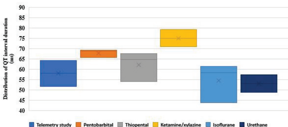
Fig. 3. Distribution of ranges of QT interval from telemetry studies and under different types of general anesthesia in male rats without accounting for light periods of the rat regimen day when the experiments were performed. Telemetry studies (n=4), pentobarbital anesthesia (n=19), thiopental anesthesia (n=8), ketamine/xylazine anesthesia (n=11), isoflurane anesthesia (n=6), urethane anesthesia (n=9), n - number of baseline or control values from which duration of QT interval was evaluated.
