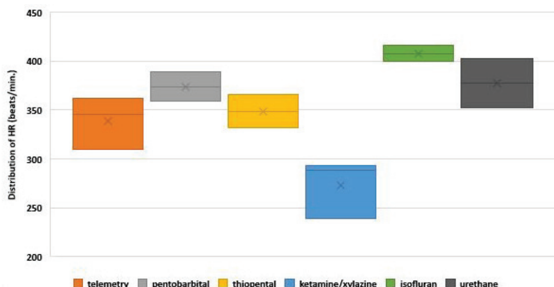
Fig. 1. Distribution of average values and ranges of heart rate (HR) from telemetry studies and under different types of general anesthesia in male rats without accounting for the light periods of the rat regimen day when the experiments were performed. Telemetry studies (n=16), pentobarbital anesthesia (n=22), thiopental anesthesia (n=13), ketamine/xylazine anesthesia (n=18), isoflurane anesthesia (n=5), urethane anesthesia (n=14), n – number of baseline or control values from which duration of PR (PQ) interval was evaluated.
