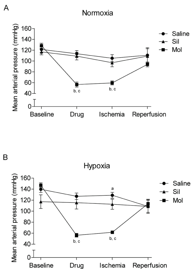
Fig. 1. Mean arterial pressure at baseline, after drug administration, at the end of 20-min coronary artery occlusion and at the end of 3-h reperfusion in normoxic (A) and chronically hypoxic (B) rats treated with saline (Saline), molsidomine (Mol) or sildenafil (Sil). Data are expressed as mean \pm SEM; n=8-11 per group. a P < 0.05 vs. corresponding normoxic group, b P < 0.05 vs. corresponding Saline group, c P < 0.05 vs. Baseline.
