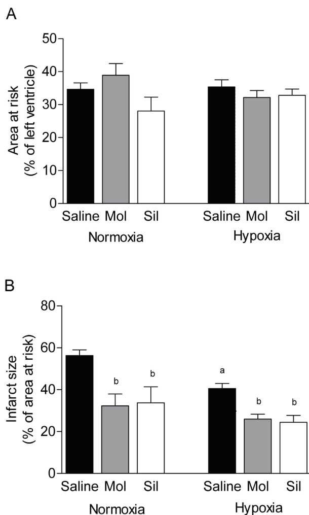
Fig. 2. Area at risk expressed as the percentage of left ventricular size ( A ) and myocardial infarct size expressed as the percentage of area at risk ( B ) in normoxic and chronically hypoxic rats treated with saline (Saline), molsidomine (Mol) or sildenafil (Sil). Data are expressed as mean \pm SEM; n=8-11 per group. a P<0.05 vs. corresponding normoxic group, b P<0.05 vs. corresponding Saline group.
