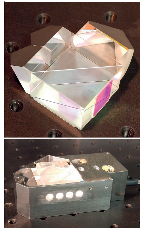
Planar differential interferometer of our design: assembled optical setup (top) mounted to the housing (bottom)
