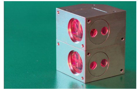
A pair of planar interferometers we developed for coordinate measurement
