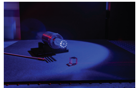
Scintillation radiation, demonstrated, is emitted from optical fibres from a scintillation crystal irradiated with ionising gamma radiation
