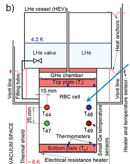
a) Experimental cryostat developed at ISI Brno for studies of RBC in a very wide range of Rayleigh numbers b) Schematic depiction of the He parts of the cryostat
