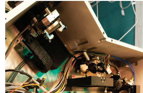
The automated gauge block calibrator based on a Dowel interferometer is capable of calibrating 100+ blocks in a single run
