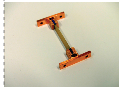
Example of an epoxy composite sample for thermal conductivity measurement in our dedicated apparatus.
