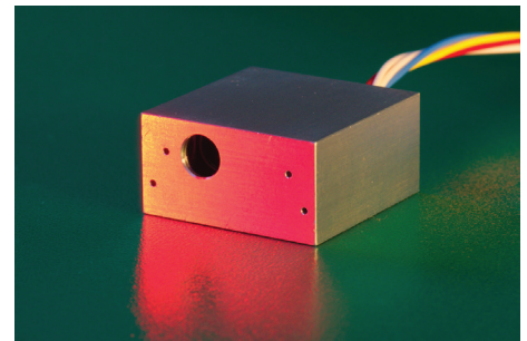
The compact homodyne receiver with four-detector arrangement of our design have proven very successful in a variety of applications
