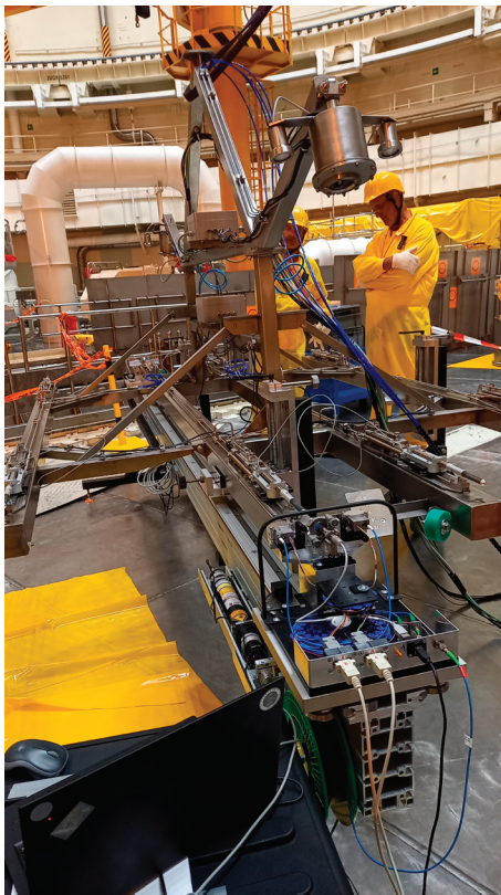
Specialized interferometric test-bench for calibration in the nuclear power plant reactor hall.
