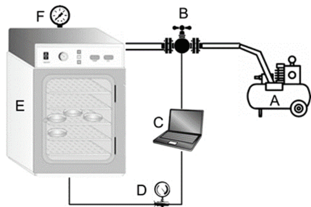
Fig. 1. Schematic graph of computer-controlled pressure cell culture system. A) Air compressor. B) Computer-controlled valve. C) Computer. D) Pressure sensor. E) Cell incubator. F) Pressure gauge.
